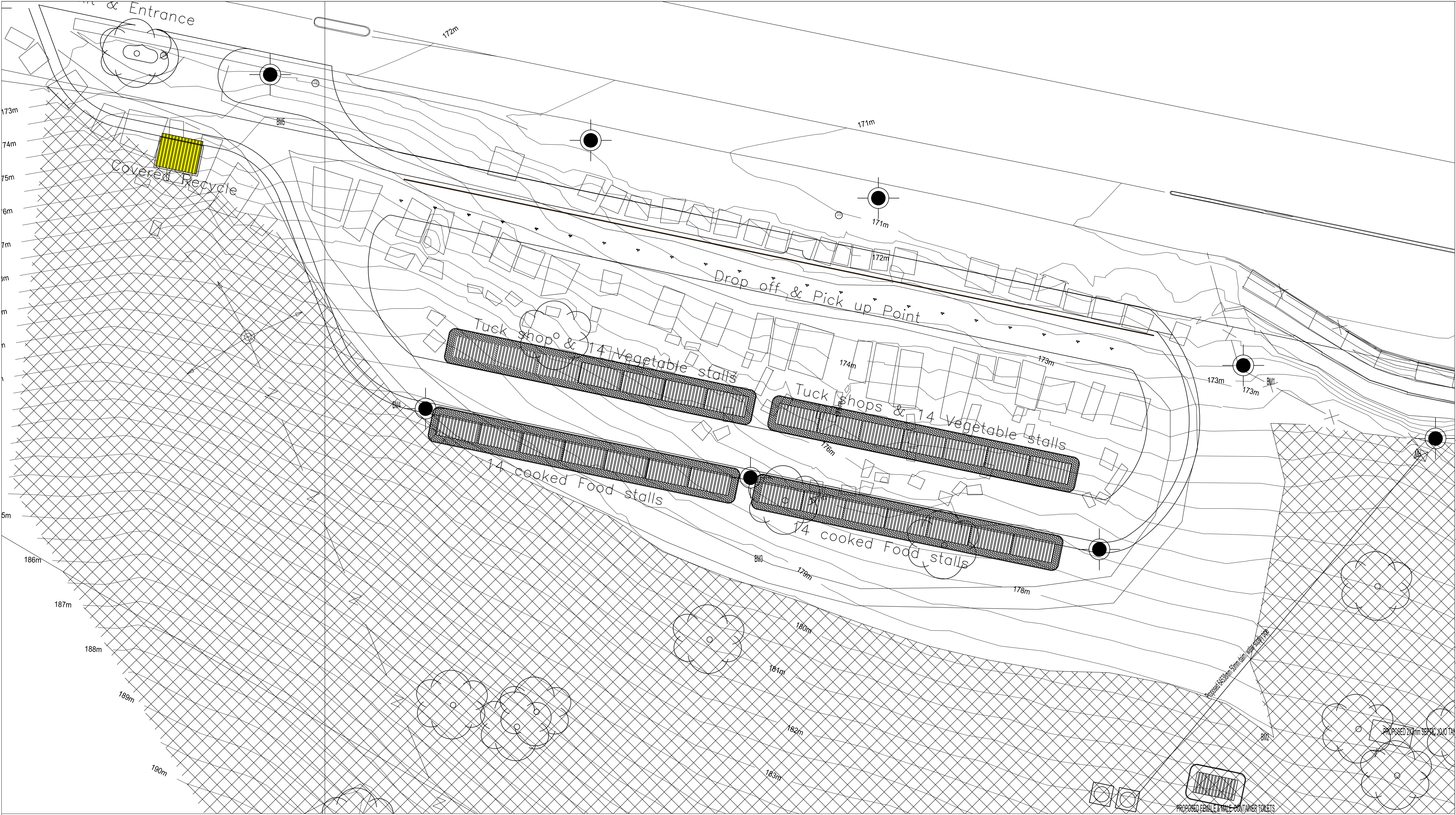
SITE DEVELOPMENT PLAN SCALE 1:300
