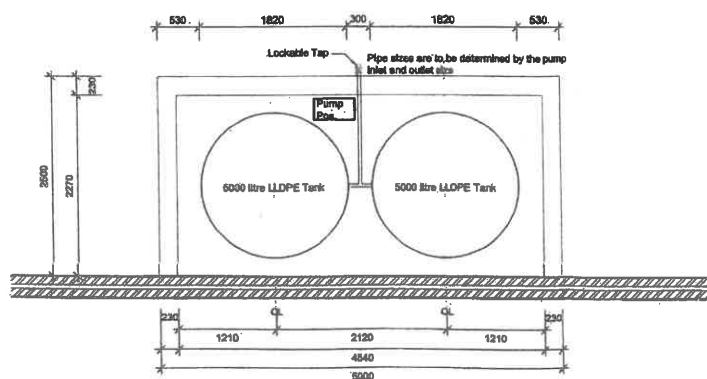
PLAN Scale 1:50
