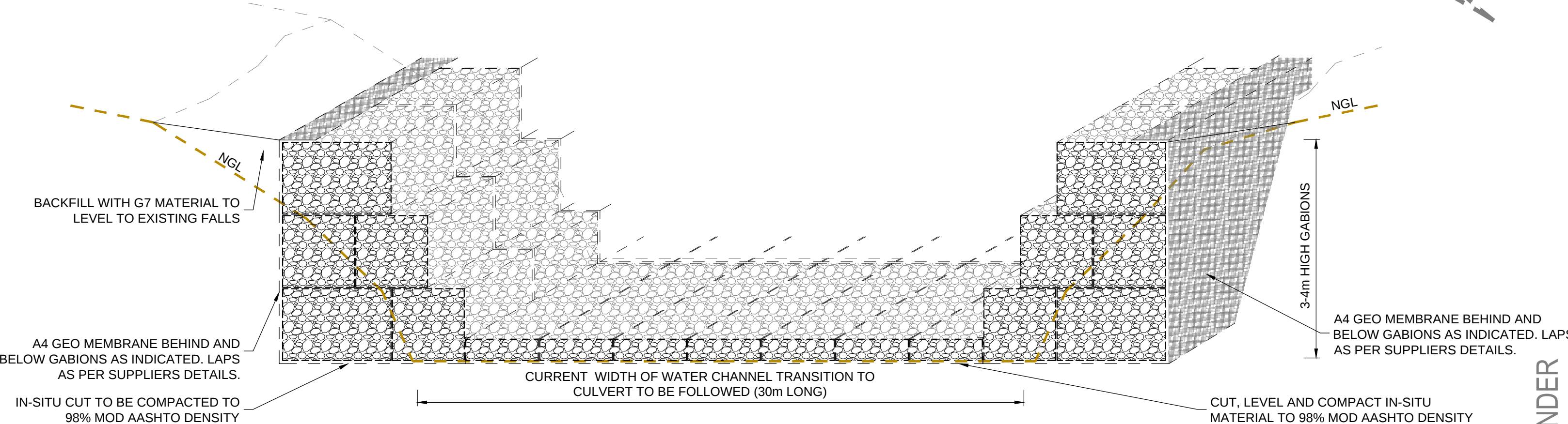
TYPICAL GABION SECTION AT ROAD STORMWATER CROSSINGS SCALE 1:50
