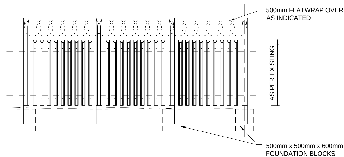
TYPICAL CONCRETE PALISADE FENCE ELEVATION SCALE 1:50
