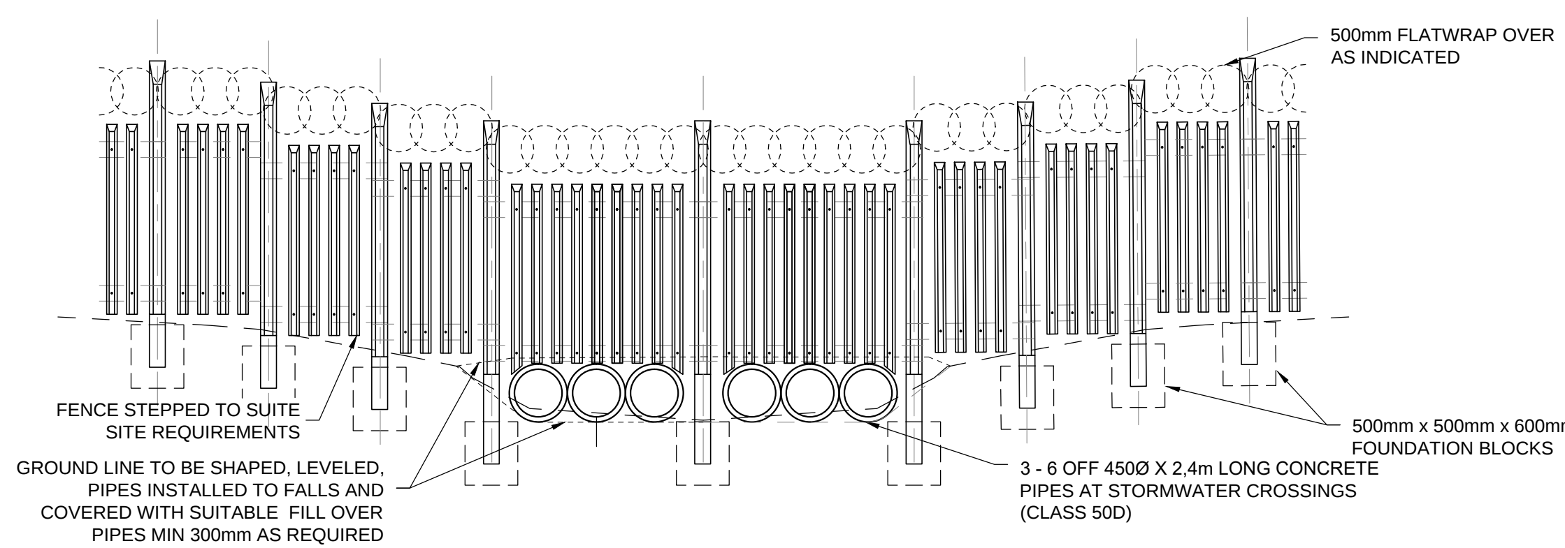
TYPICAL CONCRETE PALISADE FENCE AT STORMWATER CROSSINGS SCALE 1:50
