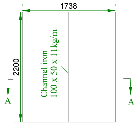
TOP VIEW : Carrier and support beams
