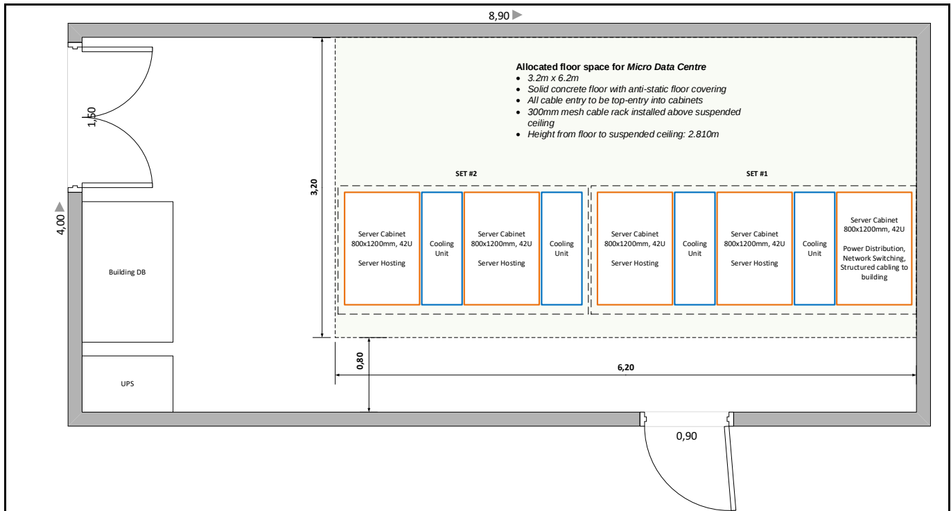
Figure 1: Server Room Layout and Dimensions (server cabinets just shown as an example of a typical layout)
