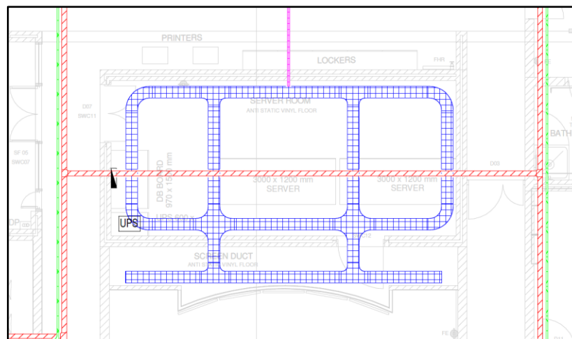
Figure 2: Mesh cable rack location in server room
