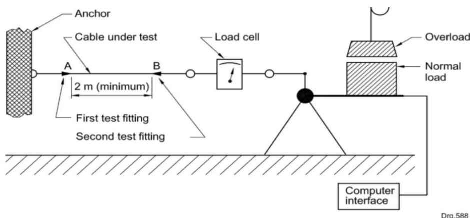
Figure: 1 – Typical arrangement for testing equipment
