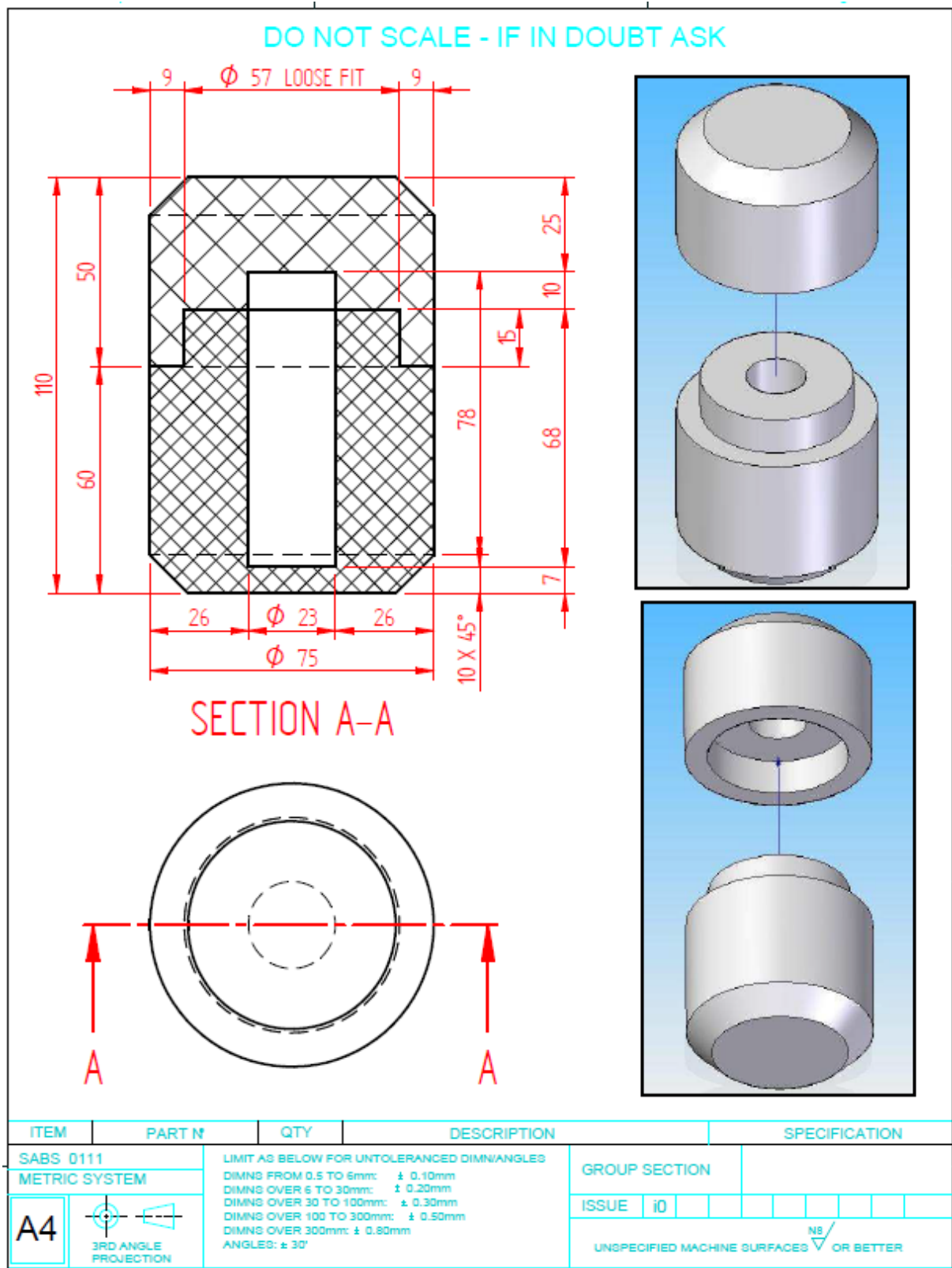
Figure 2: 75 Diameter Lead Pot Casting
