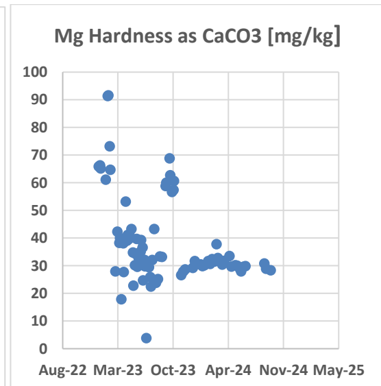
Figure 7: Raw water Mg
