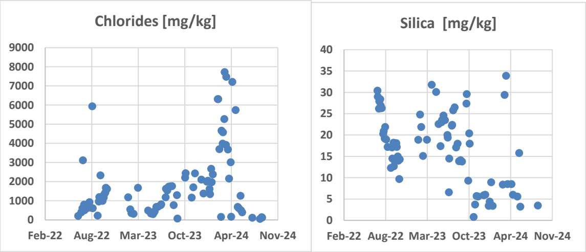
Figure 23: Dirty water recovery chlorides recovery silica
