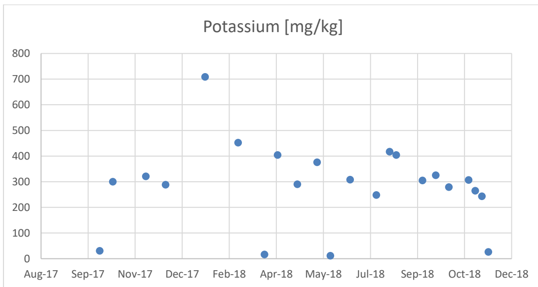
Figure 50: Tutuka SRO potassium concentration
