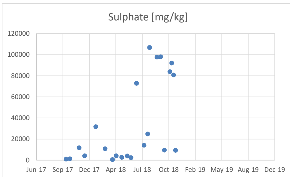
Figure 51: Tutuka SRO sulphate concentration
