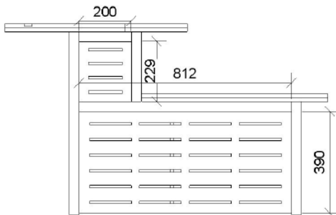
Figure 2: Console Side View with Dimensions
