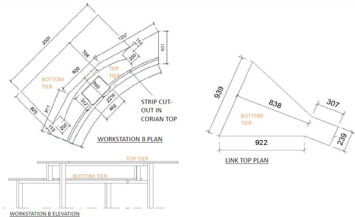
Figure 1: Console Dimensions
