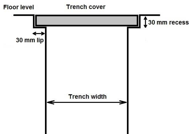
Figure 2 – Typical trench detail for item 2
