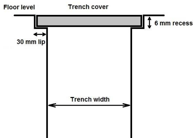
Figure 1 – Typical trench detail for item 1
