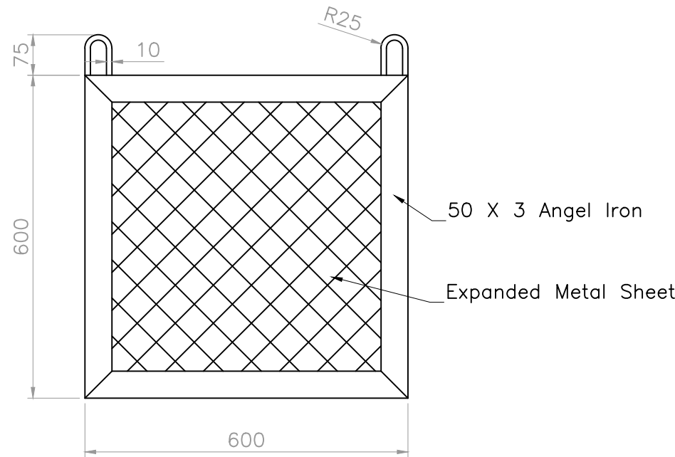
STEEL BUCKET SCALE 1:10
