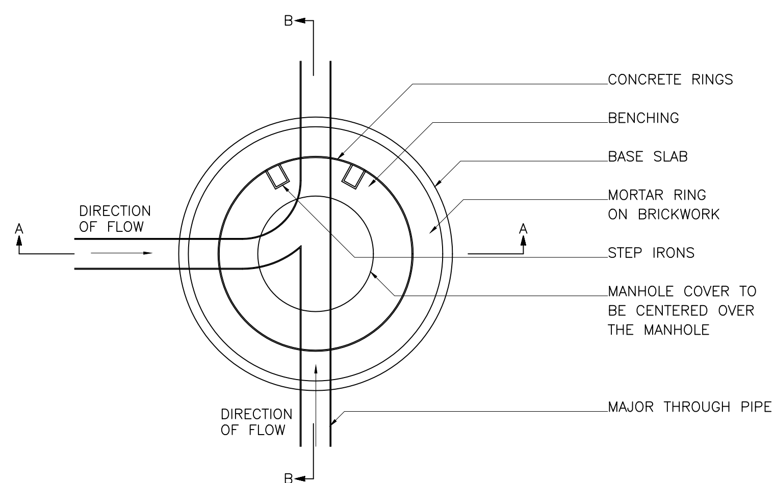
MANHOLE PLAN
