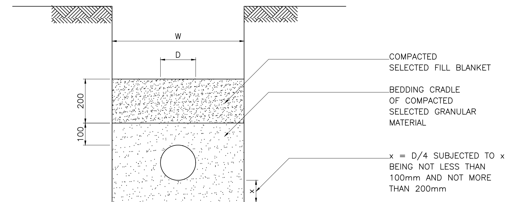
BEDDING DETAIL FOR FLEXIBLE PIPES
