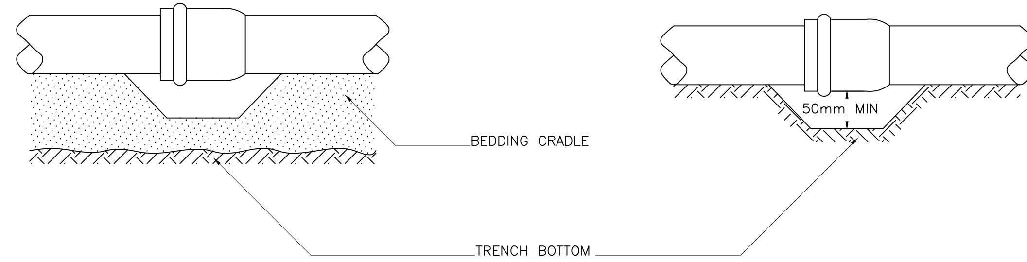
TYPICAL JOINT POCKETS FOR FLEXIBLE PIPES
