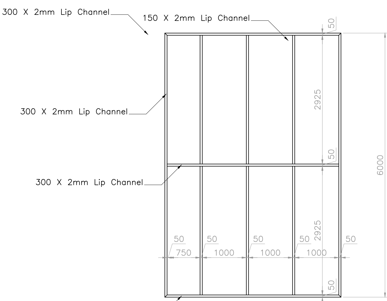
STEEL ROOF COVER SCALE 1:50
