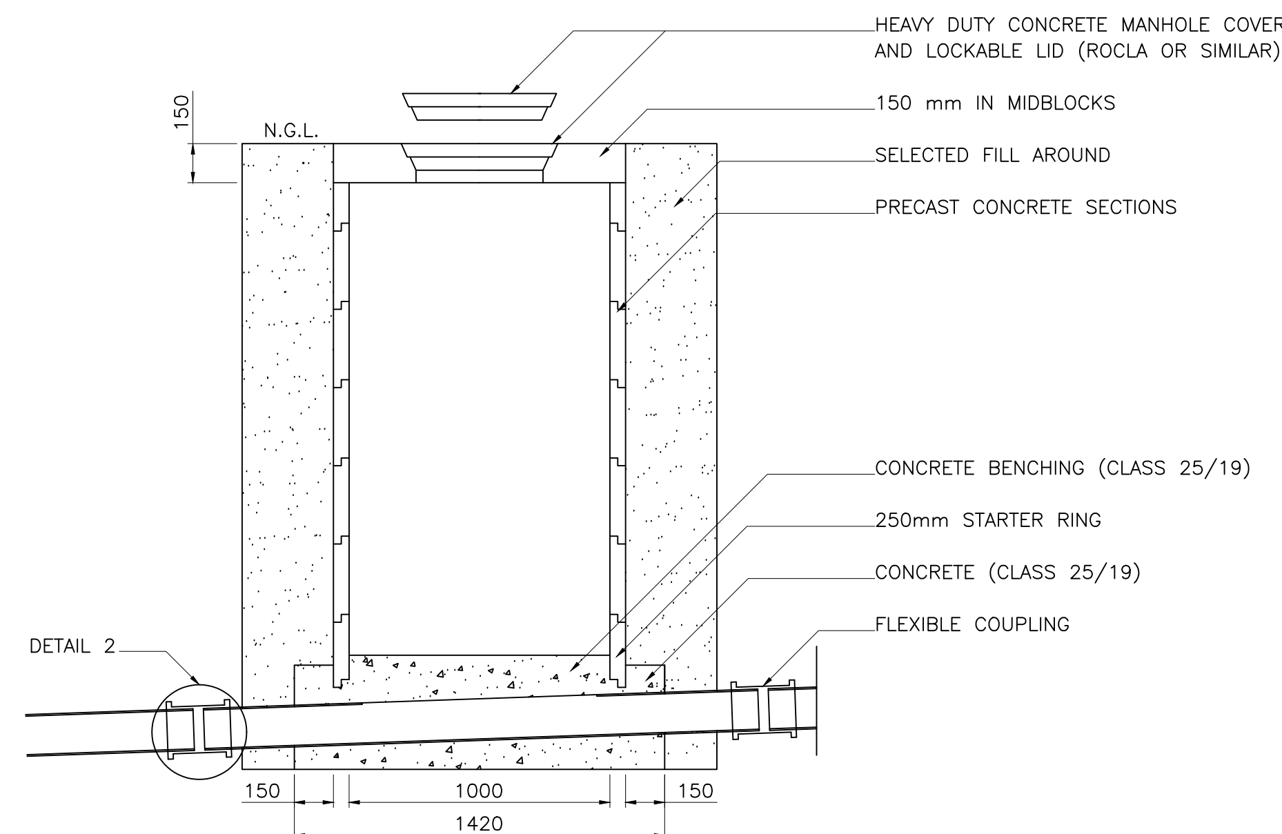
SECTION B-B
