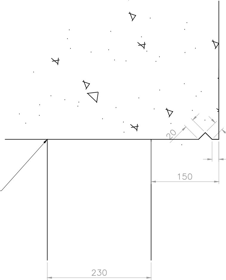
CONCRETE ROOF DETAIL SCALE 1:5
