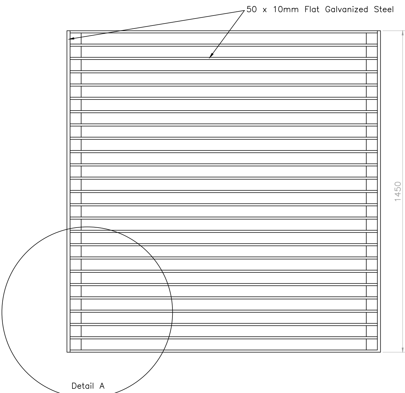
GALVANIZED RAKE SCREEN SCALE 1:10
