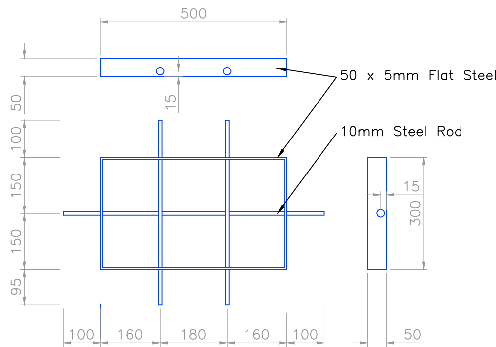
STEEL WINDOW GRID SCALE 1:10
