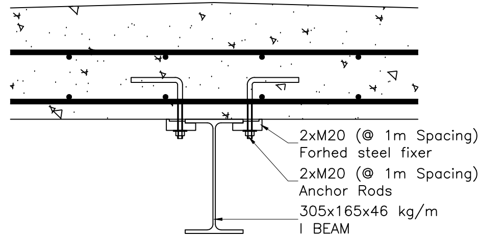
I BEAM FIXING DETAIL SCALE 1:10
