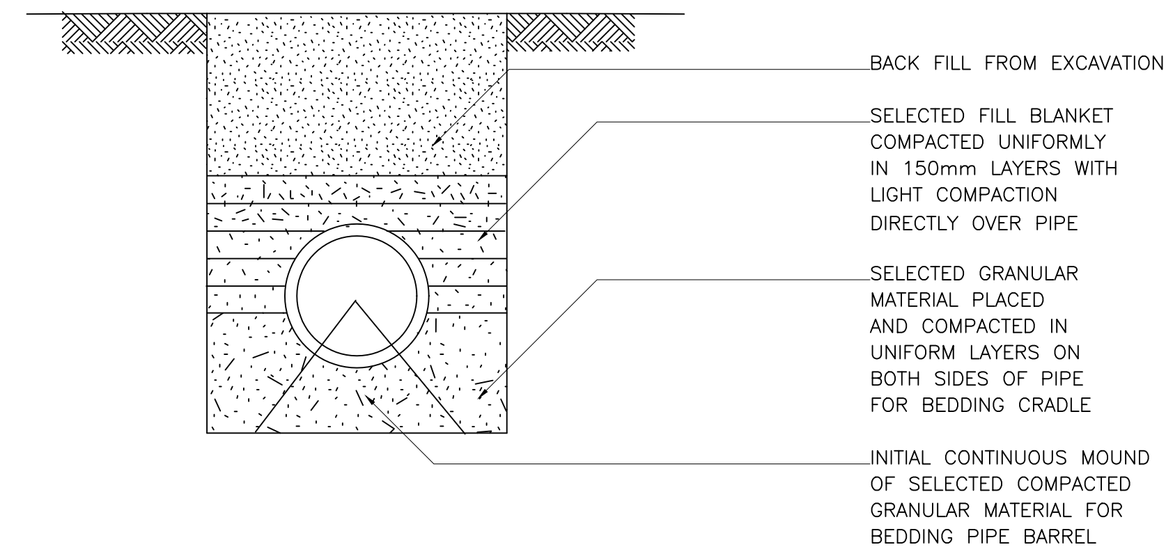
FLEXIBLE PIPE SUPPORTED ON SELECTED GRANULAR MATERIAL CONSTRUCTION METHOD OF PIPE BEDDING
