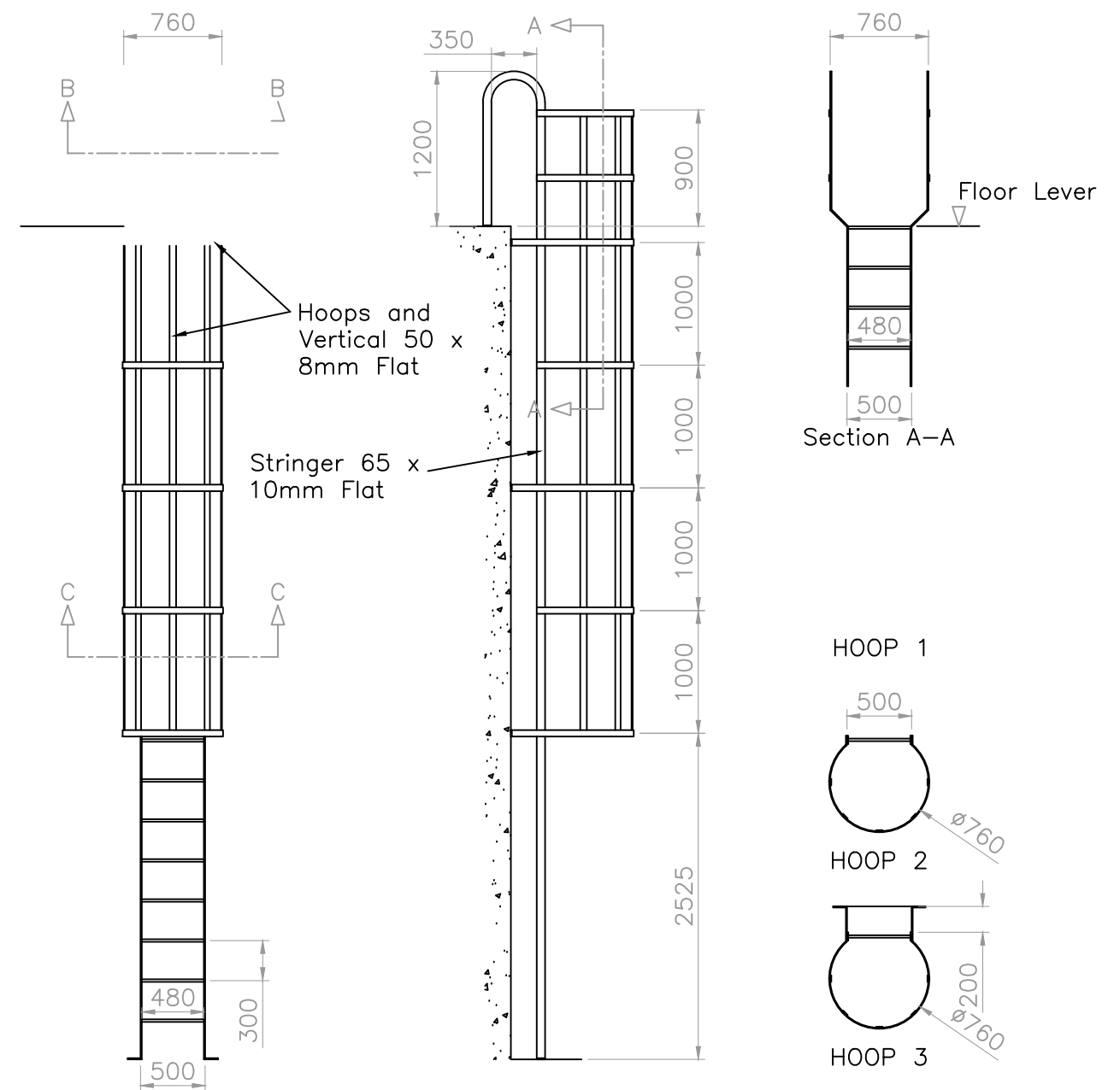
GALVANIZED VERTICAL LADDER SCALE 1:50
