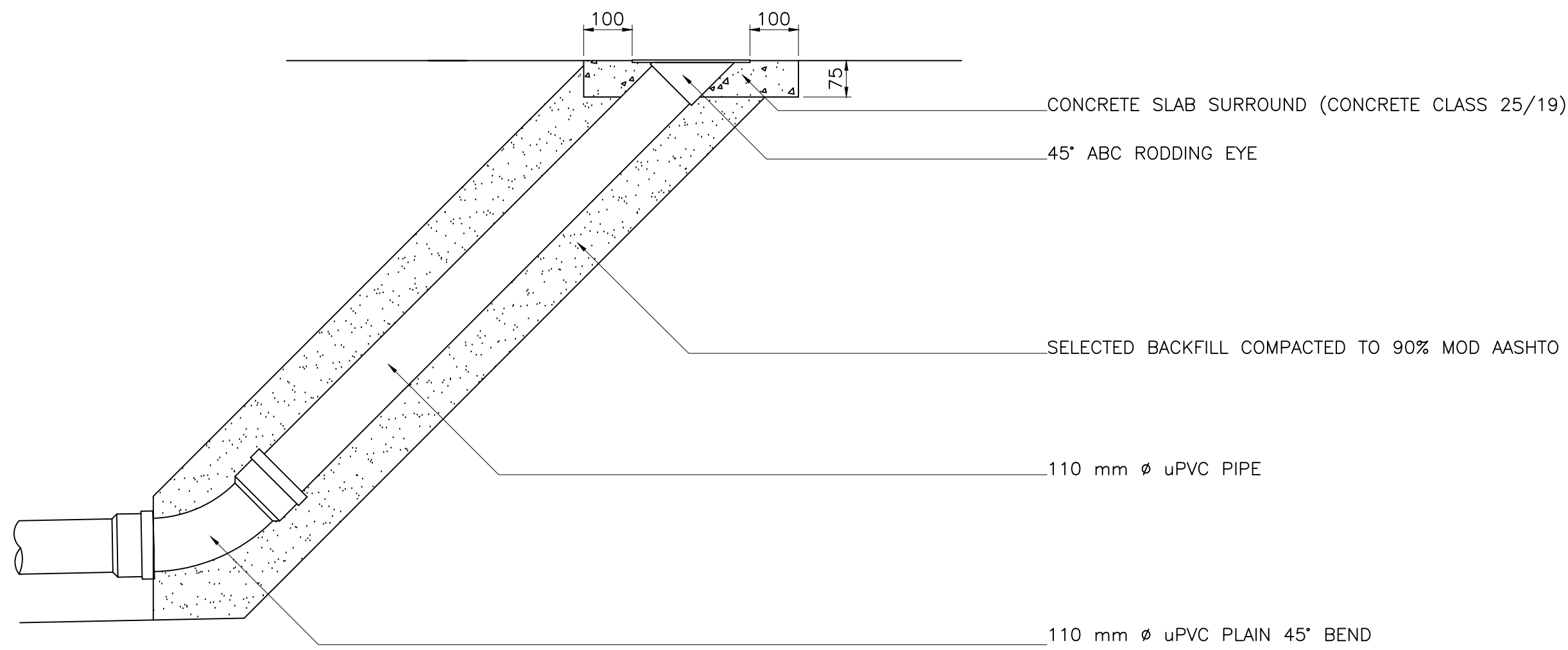
TYPICAL DETAIL OF RODDING EYE AT THE HEAD OF THE ERF SEWER LINE
