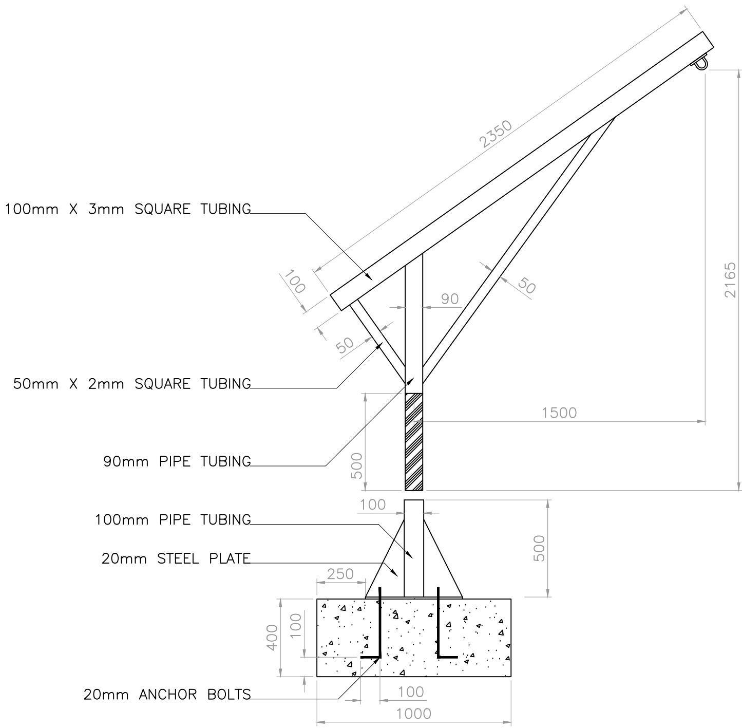
SWIVEL LIFTING DAVIT SCALE 1:20
