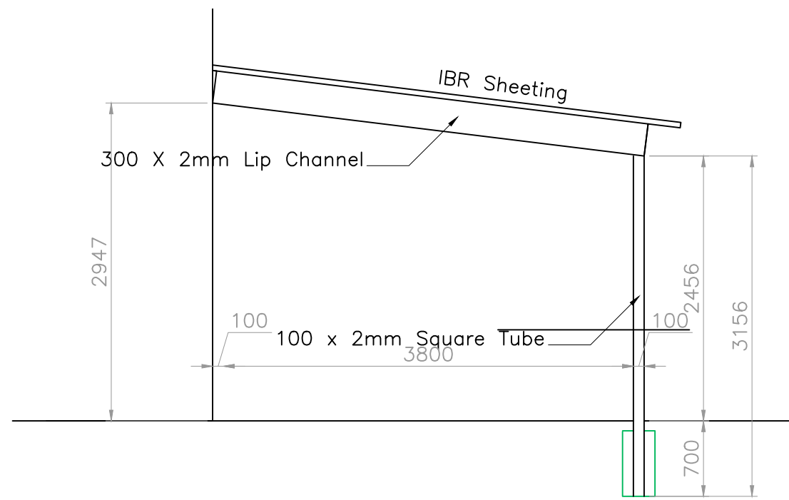
STEEL ROOF COVER SCALE 1:50
