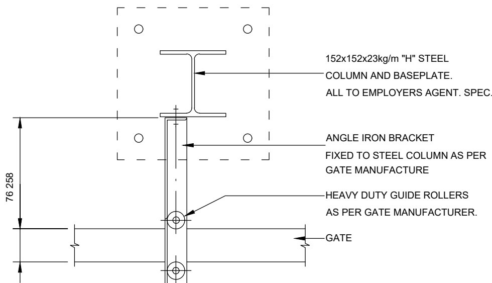
DETAIL 2 - PLAN SCALE 1:10
