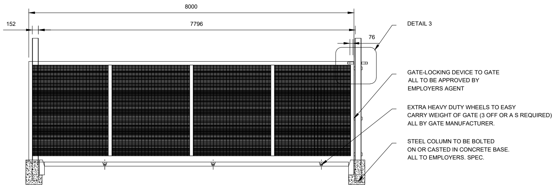
TYPICAL SLIDING GATE: ELEVATION SCALE 1:50
