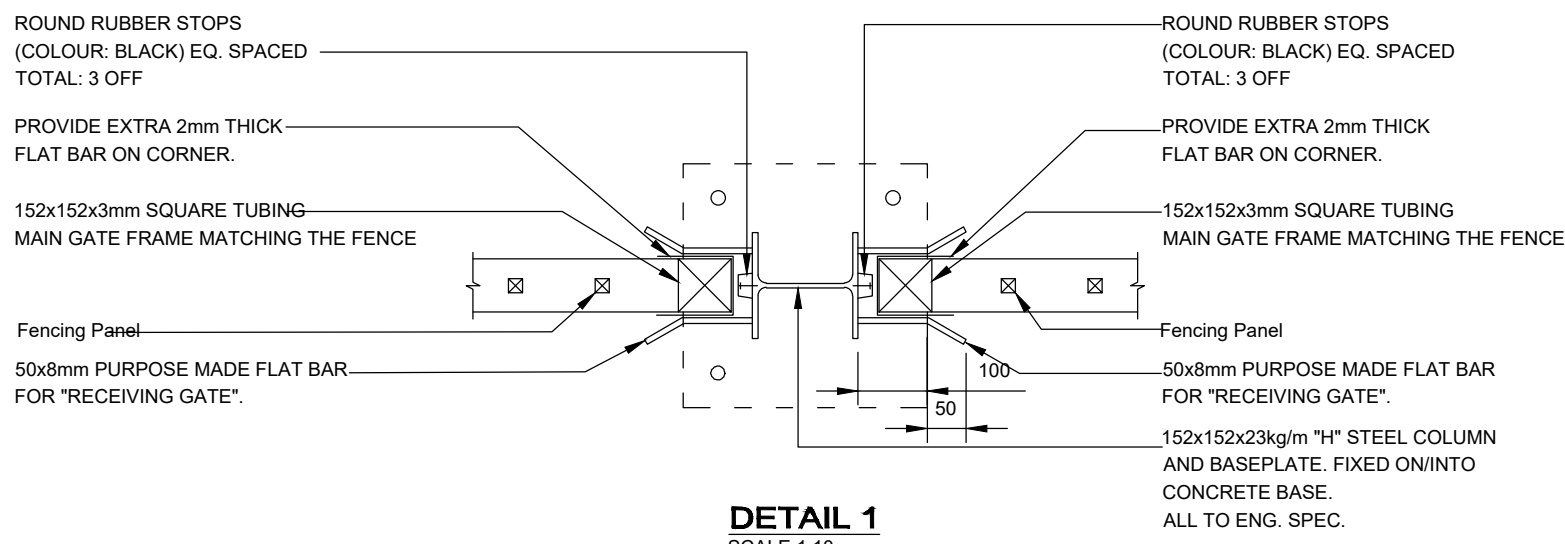
DETAIL 1 SCALE 1:10
