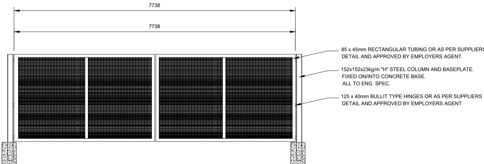
TYPICAL DOUBLE SWING GATE: ELEVATION SCALE 1:50
