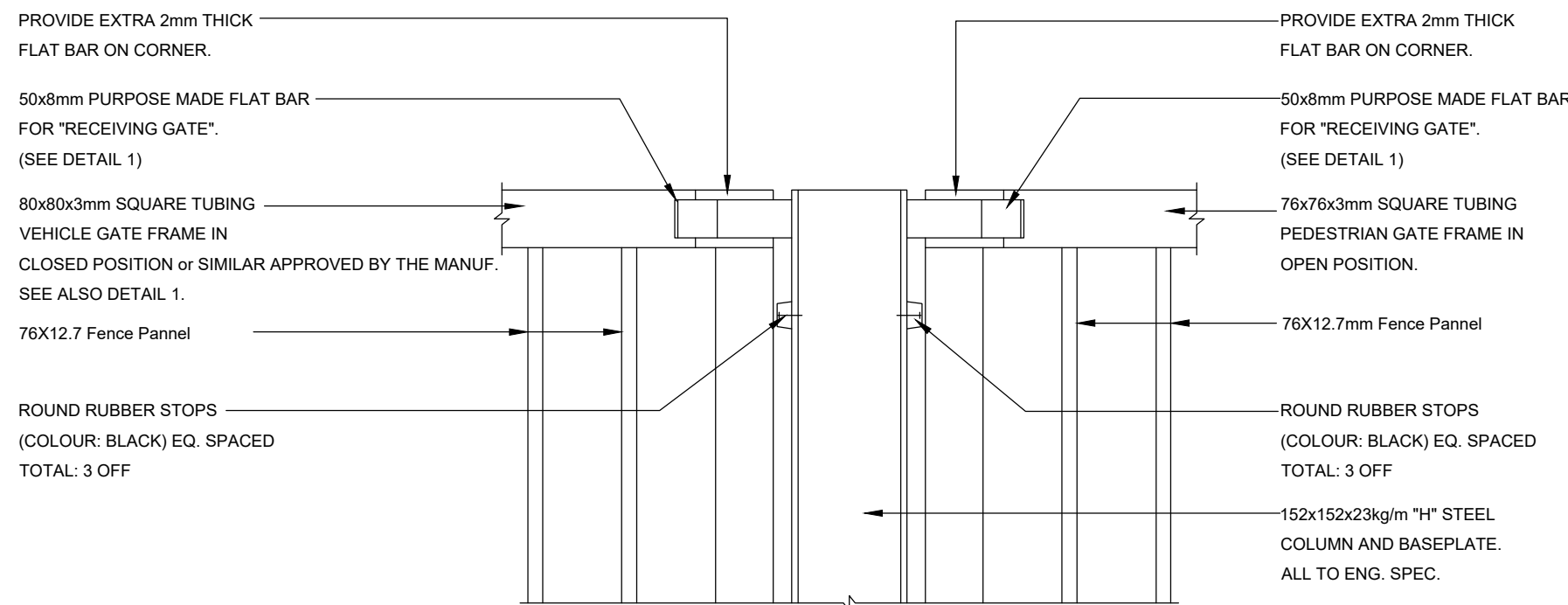
DETAIL 3 - ELEVATION SCALE 1:10
