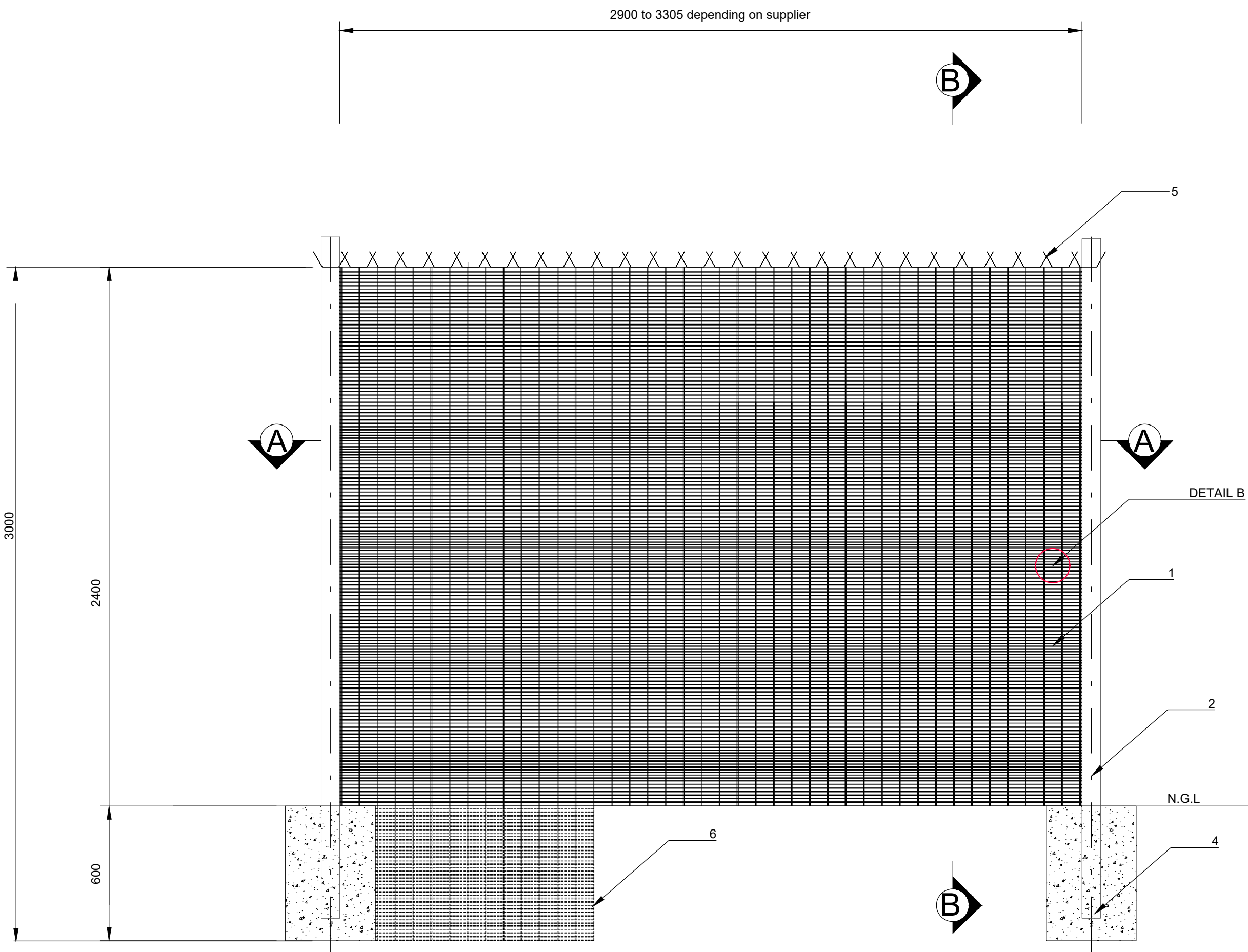
FRONT ELEVATION SCALE 1:20
