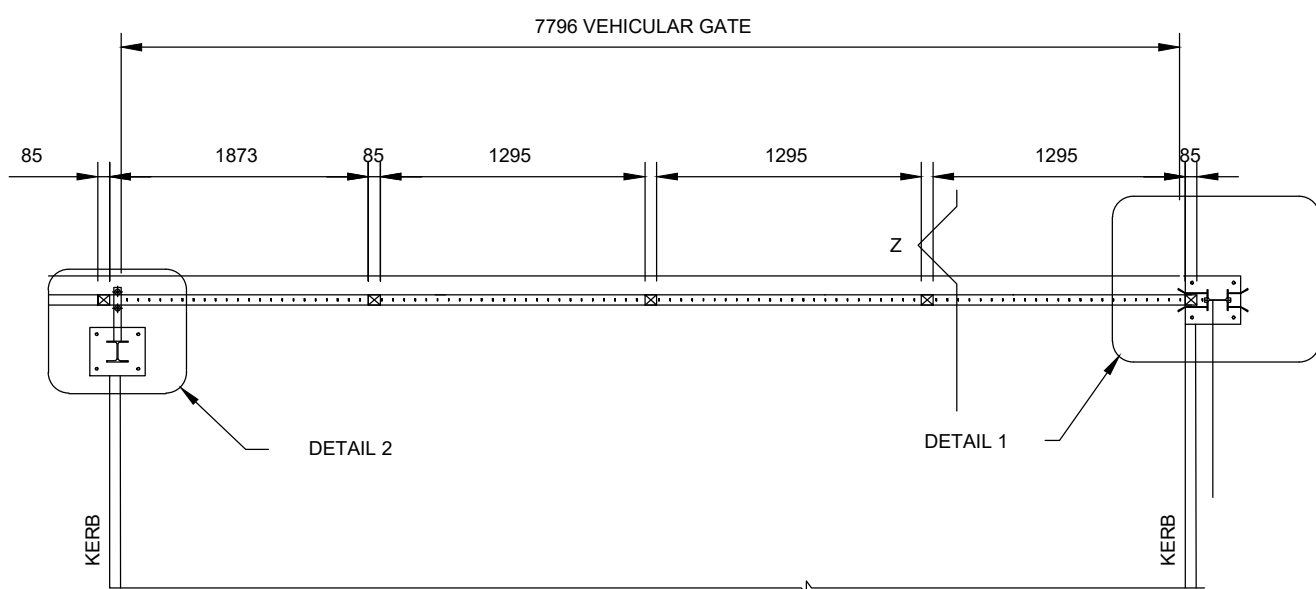
VEHICLE AND PEDESTRIAN GATE PLAN SCALE 1:50
