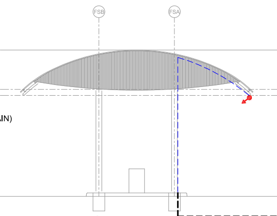
EAST ELEVATION FILLING STATION Scale 1 : 100
