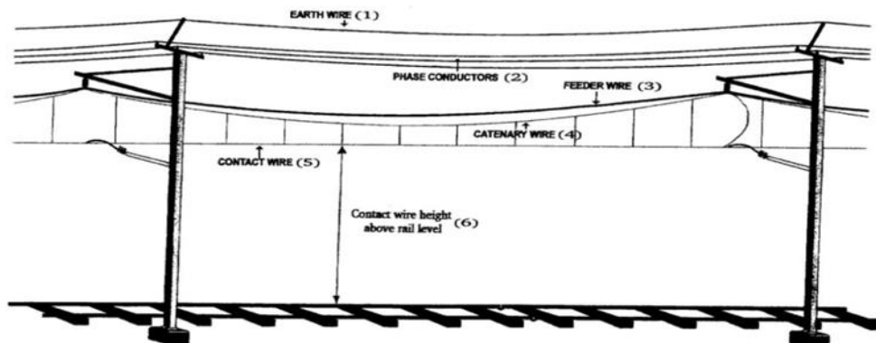
Figure 1: O.H.T.E Layout
