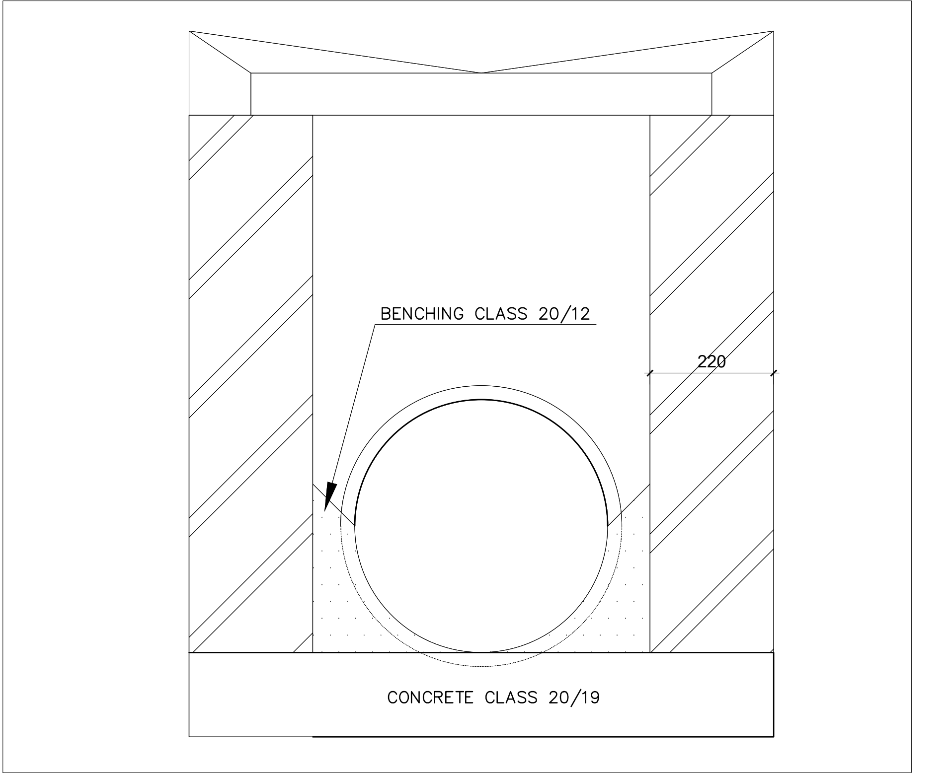
TYPICAL PIPE SECTION N.T.S
