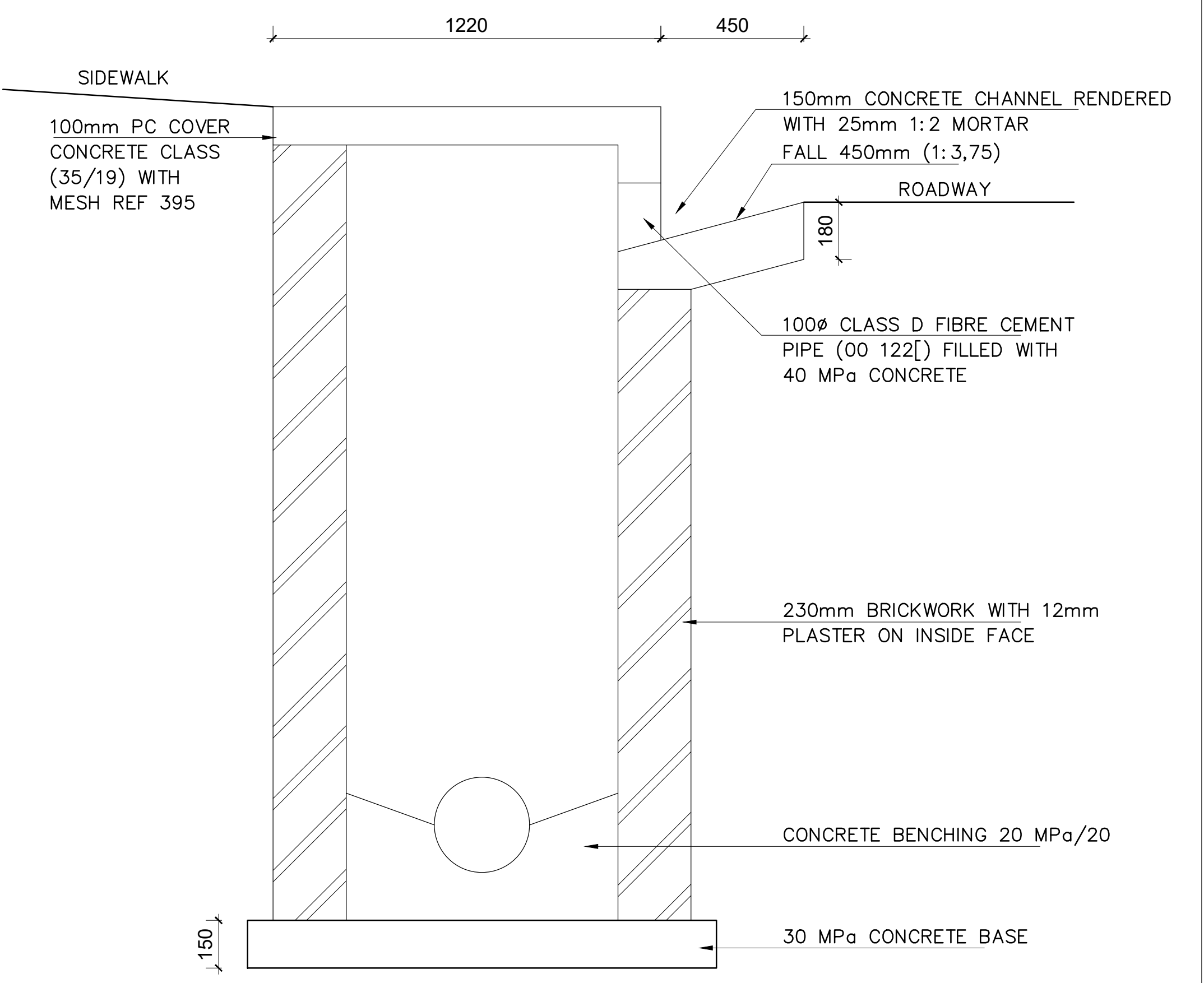
SECTION THROUGH KERB INLET N.T.S
