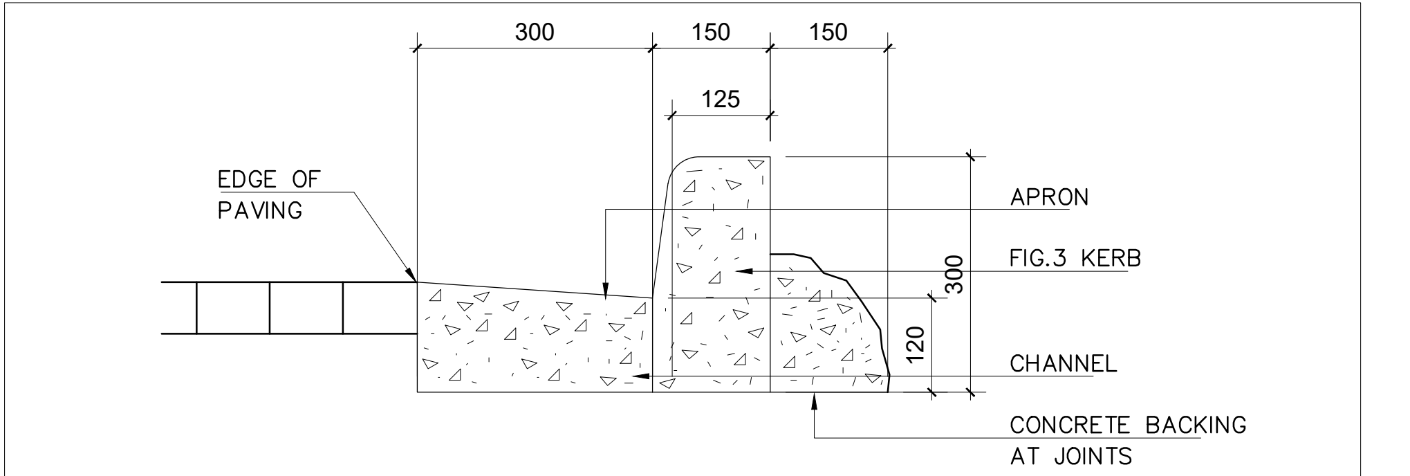
DETAIL OF BARRIER KERB N.T.S
