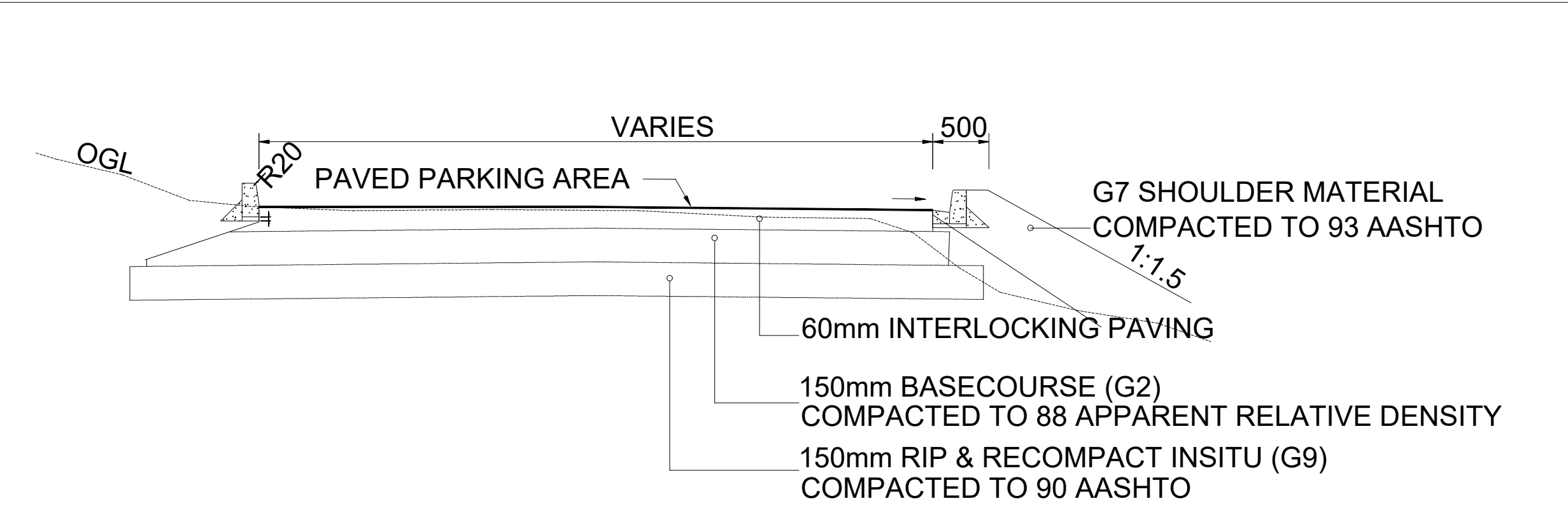
PARKING AREA CROSS SECTION N.T.S
