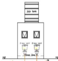
NORTHERN ELEVATION Scale 1:100
