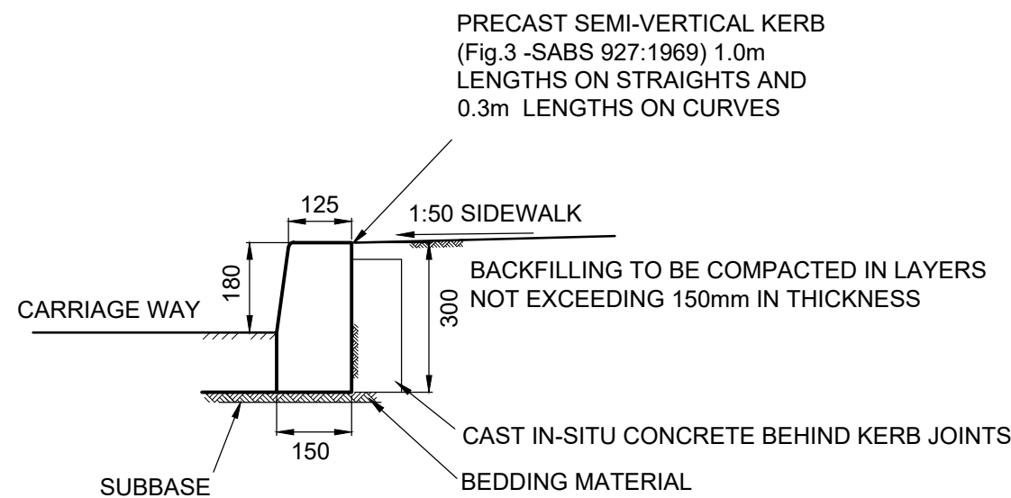
BARRIER KERB (FIG. 3 - SABS 927:1969) SCALE 1:20
