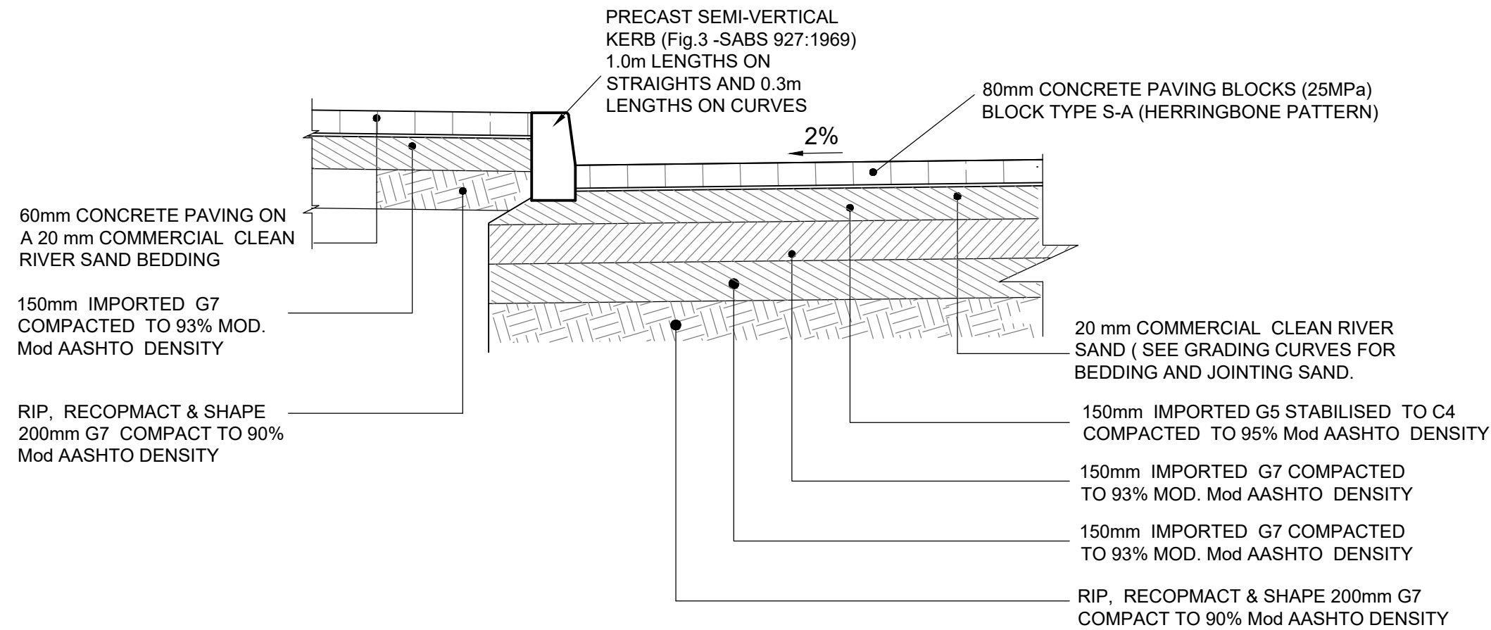
TYPICAL ROADS & PARKING SECTION SCALE 1:20
