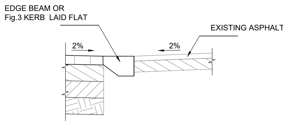
EDGE BEAM DETAIL SCALE 1:20
