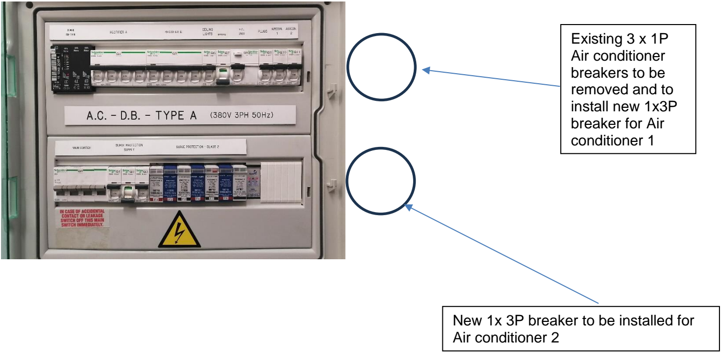
Figure: Existing AC Board
