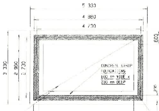
Fuel Stores Floor Plan
