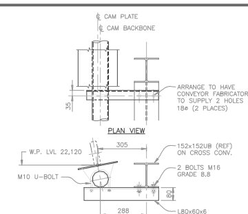
SECTION A-A CAM SUPPORT OVER CROSS CONVEYOR SCALE:- 1:10
