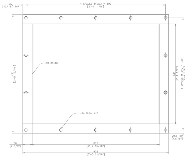
32" RECTANGULAR STANDARD FLANGE
