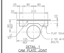
DETAIL 1 CAM PLATE JOINT SCALE:- 1:5
