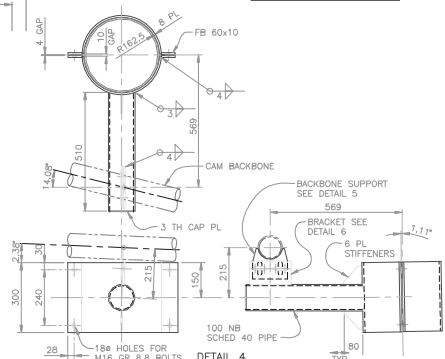
DETAIL 4 SCALE = 1:10
