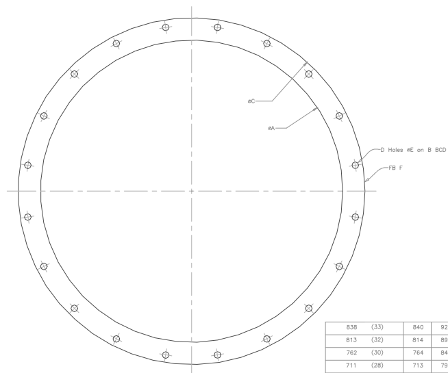
ROUND STANDARD FLANGE
