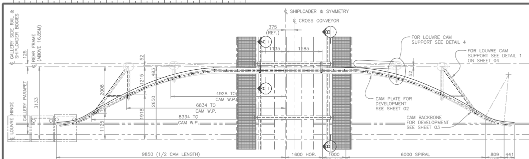
PLAN VIEW - LOUVRE CAM
