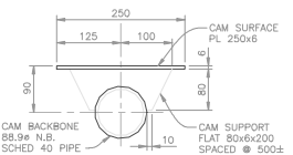
DETAIL 3 CAM PLATE SUPPORT SCALE: = 1:5
