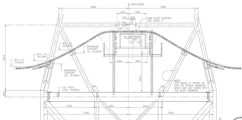
SIDE VIEW - LOUVRE CAM
