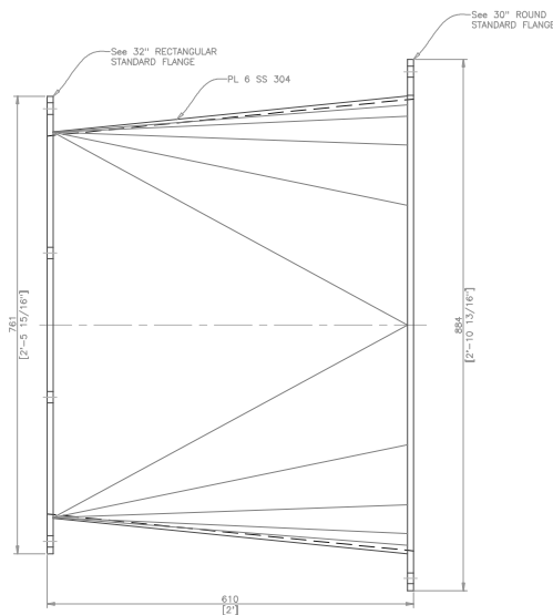
RECTANGULAR FLANGE TO ROUND FLANGE TRANSITION
