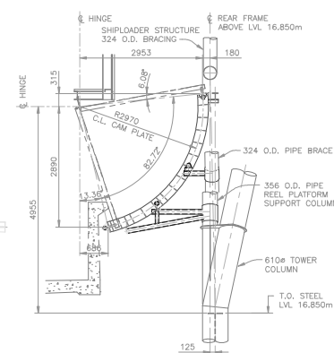
END VIEW - LOUVRE CAM
