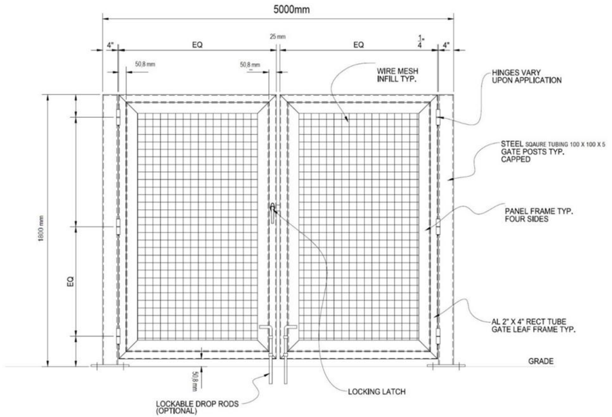
ELEVATION VIEW
