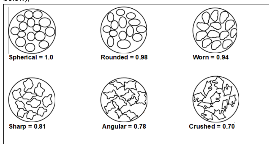
Figure 1: Typical grain shape of sphericities of granular fine filter sand.
