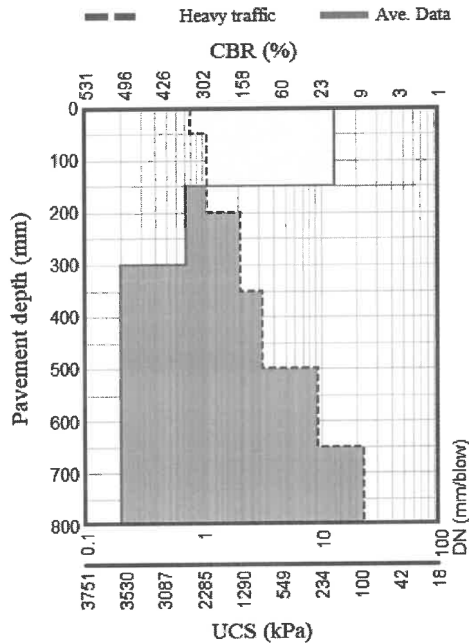
Layer Strength Diagram (LSD)(Existing Structure)
