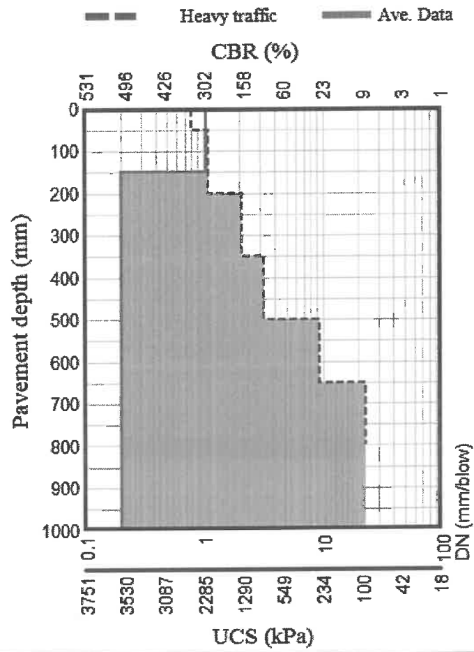
Layer Strength Diagram (LSD)(Existing Structure)
