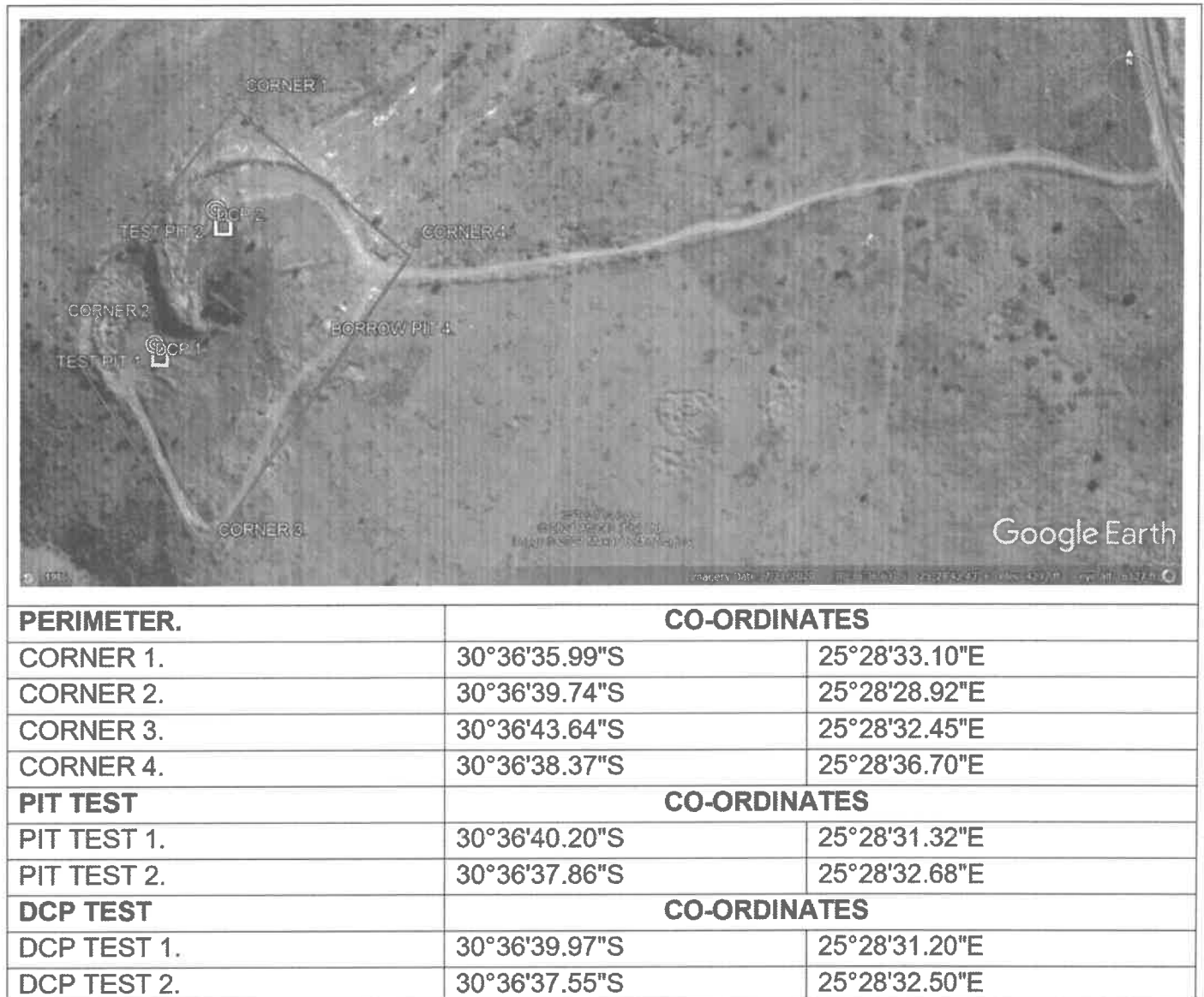
Figure 9. Indicating the dimensional boundary by GPS co-ordinate of borrow pit one as well as points of the pit test and DCP test.
