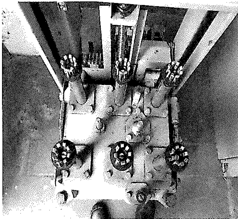
Image B.2.4 - Main isolating contactors of OCB
