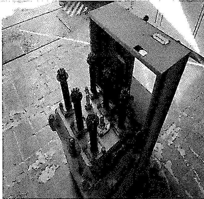
Image B.1.4 - Inside existing switchgear
