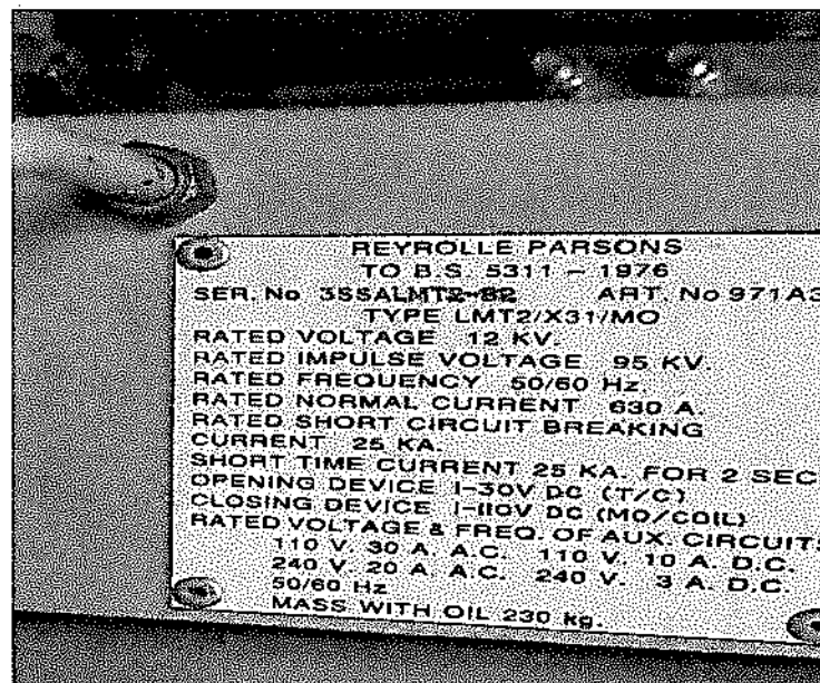
Image B.1.2 - Nameplate
