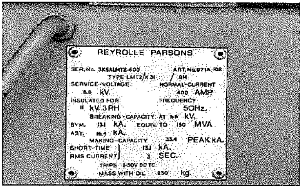
Image B.3.3 - Breaker nameplate
