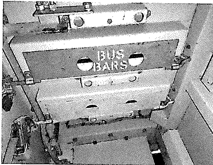
Image B.4.2 - Shutters
