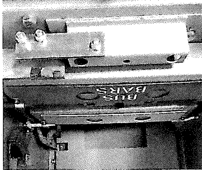
Image B.1.6 - Shutter operating mechanism
