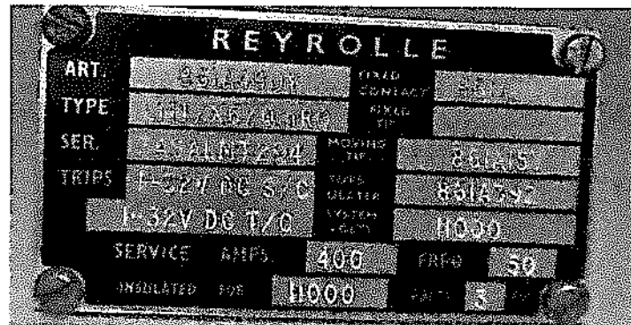
Image B.5.1 - Nameplate
