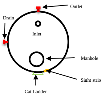
Figure 1: Sodium Hypo Storage Tank
