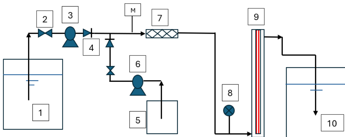
Figure 1: Process Flow Diagram of UV/chlorine process (1) Influent tank; (2) ball valves; (3) Influent pump; (4) non-return valve; (5) Chemical tank; (6) chemical dosing pump; (7) Mixer; (8) Sampling point; (9) UV reactor; (10) Effluent tank; (M) Flow meter.
