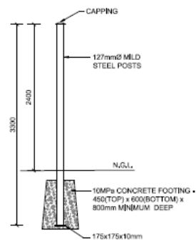
INTERMEDIATE STRAINING POSTS (SINGLE POSTS)
