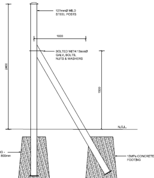
TYPICAL MAIN POST STAY
