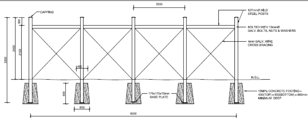
MAIN STRAINING BOXES (FIVE POSTS)
