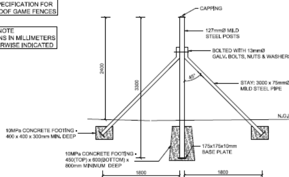
STRAINING POSTS (SINGLE POSTS)
