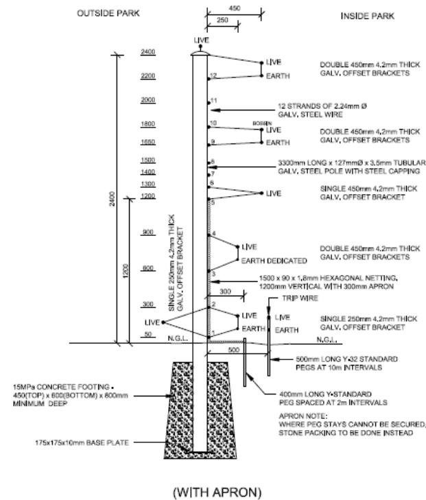
ELECTRICAL FENCING 1:25
