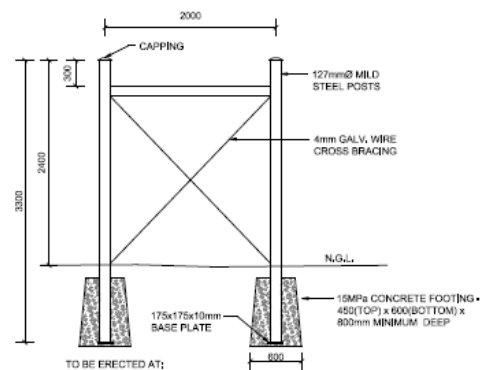
DOUBLE STRAINING BOXES (DOUBLE POSTS)
