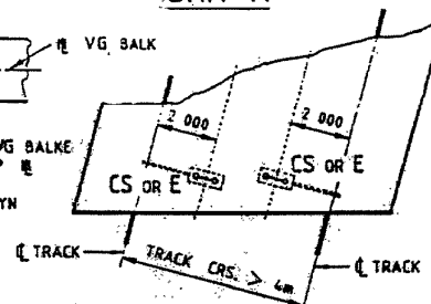
PLAN 'B' (TRACK CRS. > 4\text{m} ) (FURTHER DETAILS AS FOR PLAN 'A')
