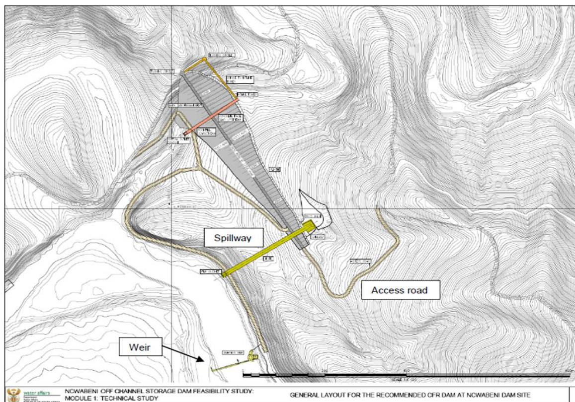
Figure 2: Proposed Cwabeni Off-Channel Storage Dam Project layout.
