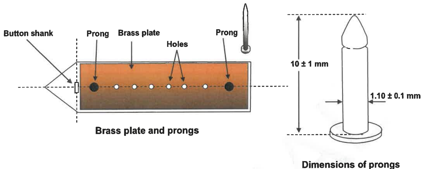
Figure 6 – Prongs and brass plate
