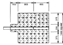
FOOTING DETAIL FOR SANDY CONDITIONS
