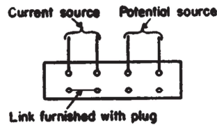
Fig. 18. Plug connection for Fig. 16 for testing one current and one potential coil with separate source
