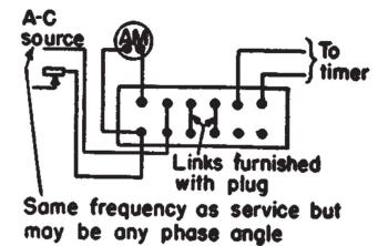
Fig. 22. Plug connection for Fig. 19 for testing relay with same or separate source
