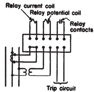
Fig. 19. Test-block connection for one current and one potential coil with connection for trip circuit
