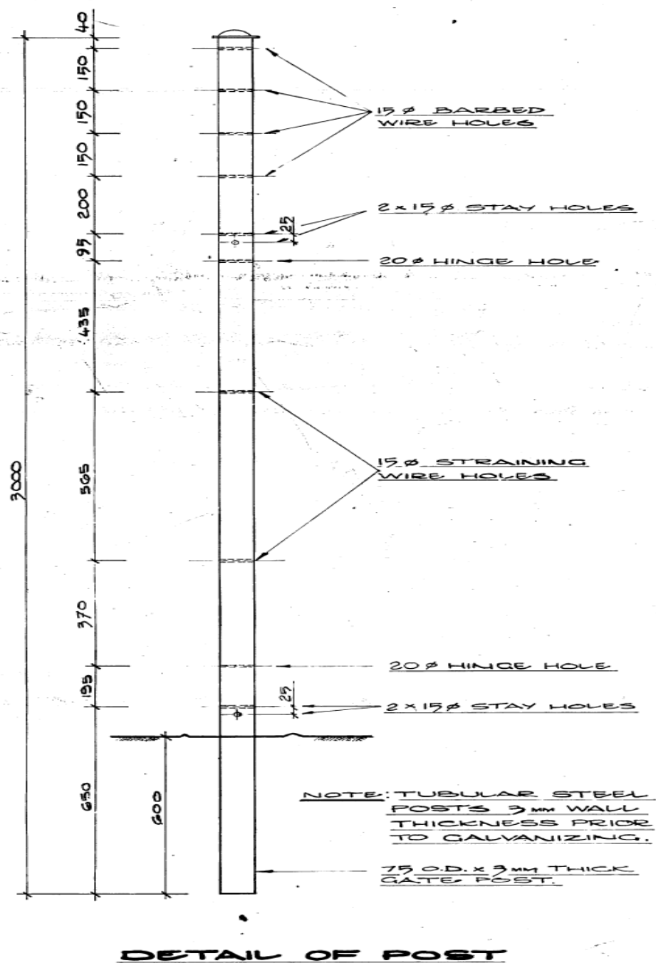
Figure 2. Item 21 - Drawing: PRA 2080 Rev 6
