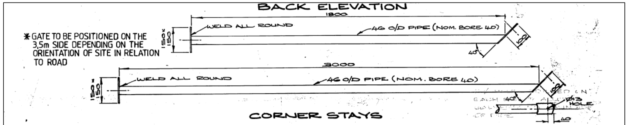
Figure 3. Item 26 and 27 -Drawing: PRA 2080 Rev 6
