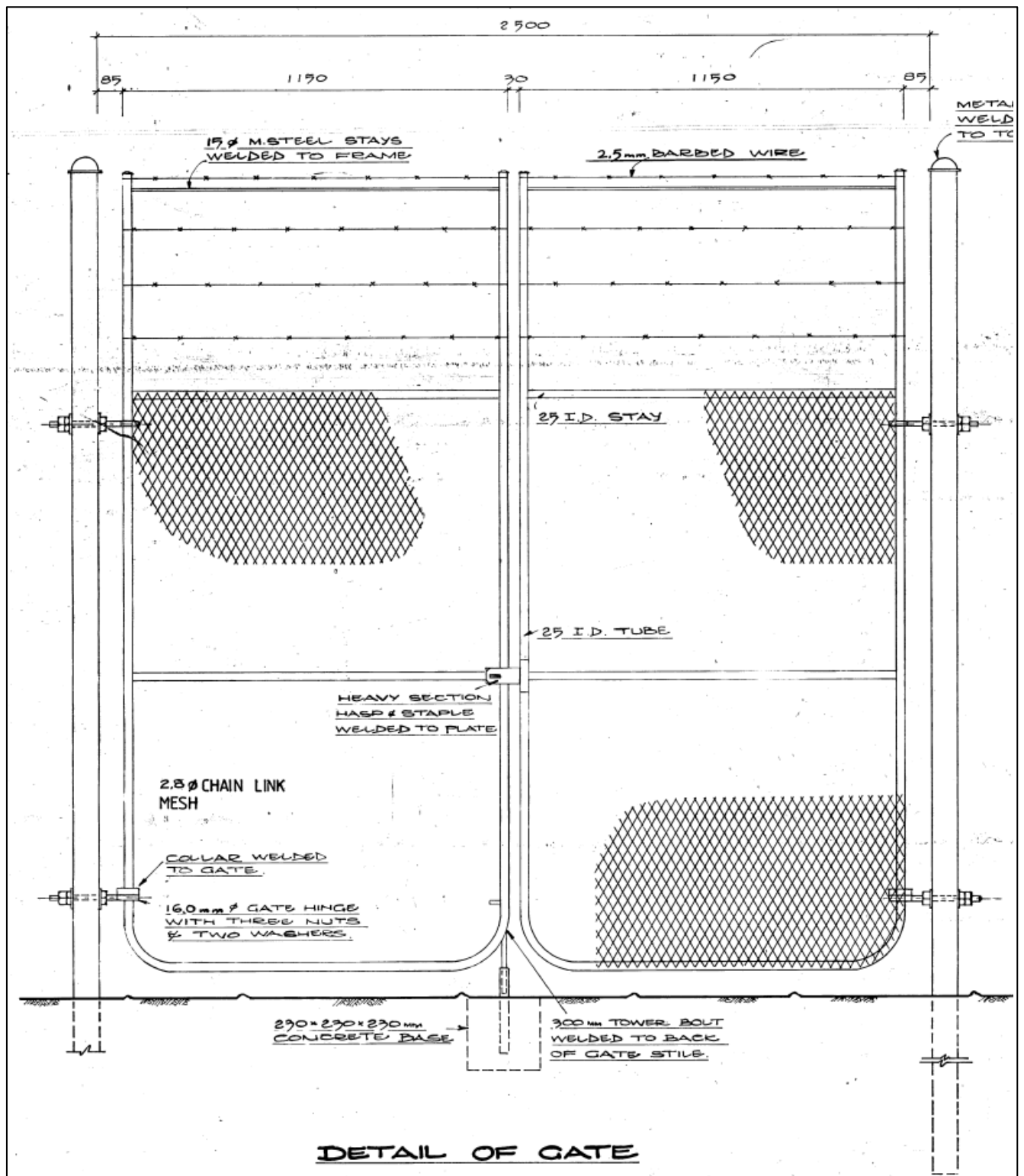
Figure 6. Item 55 (LHS) and 56 (RHS) - Drawing: PRA 2080 Rev 6
