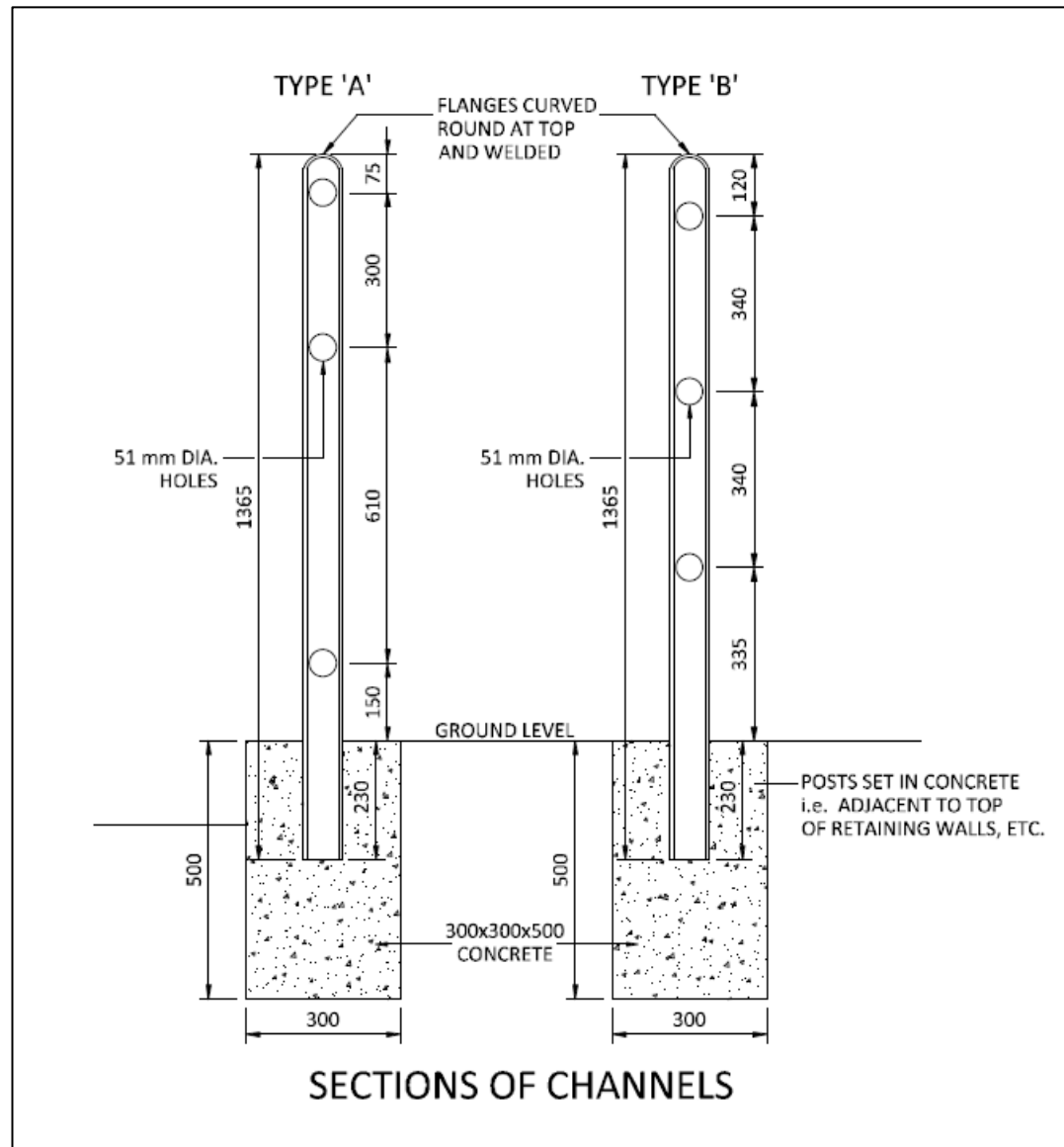
Figure 1 . Item 19 and 20 - Drawing:R26B_FEB 2013
