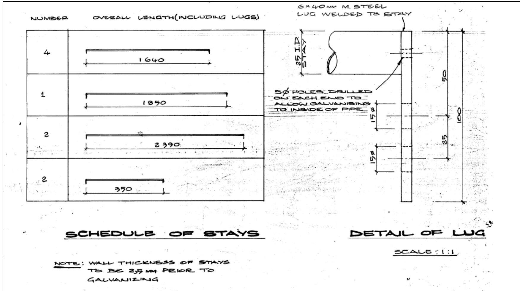
Figure 4. Item 31, 32 and 33 - Drawing: PRA 2080 Rev 6
