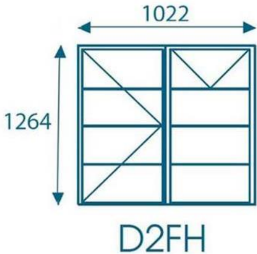
Figure 5. ITEM 47 - Illustration of D2FH window frame
