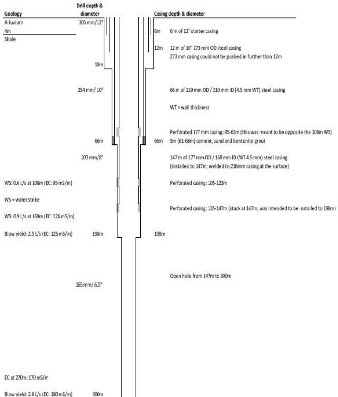
Figure 5. GWA1 construction
