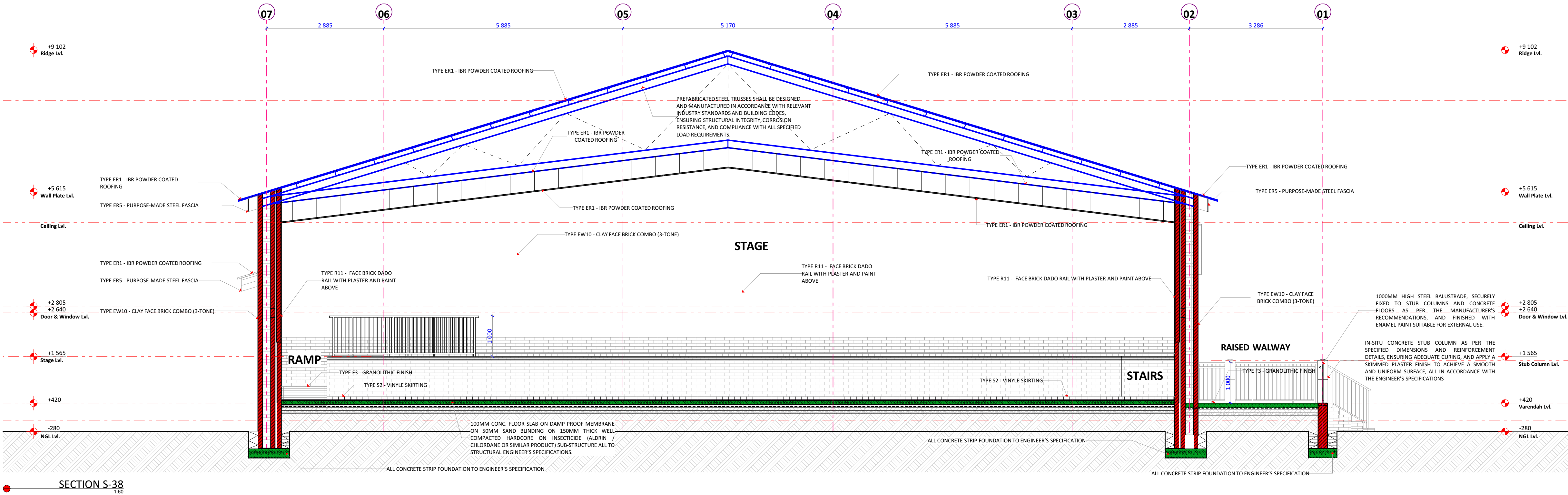
SECTION S-38 1:80
