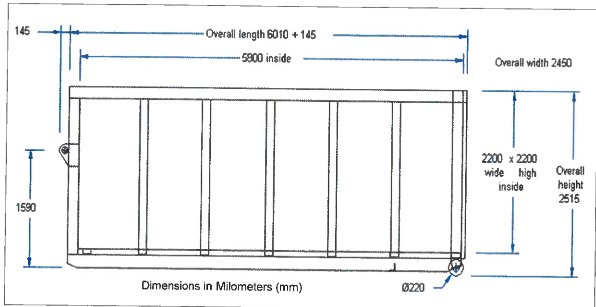
Diagram: 28m 3 Bulk Waste Container
