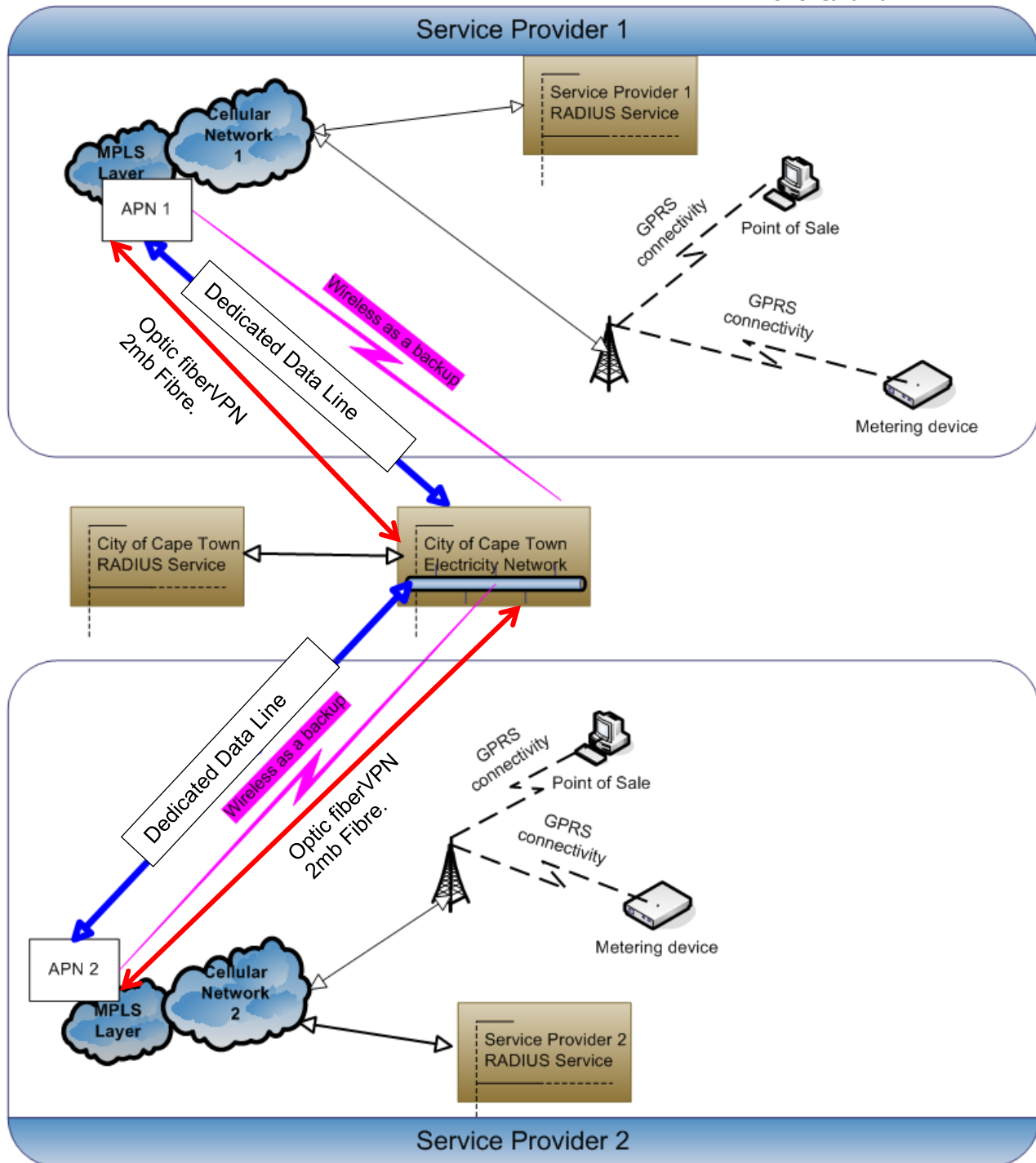
Figure 2. Secure GPRS/3G Services from more than one Cellular Provider
