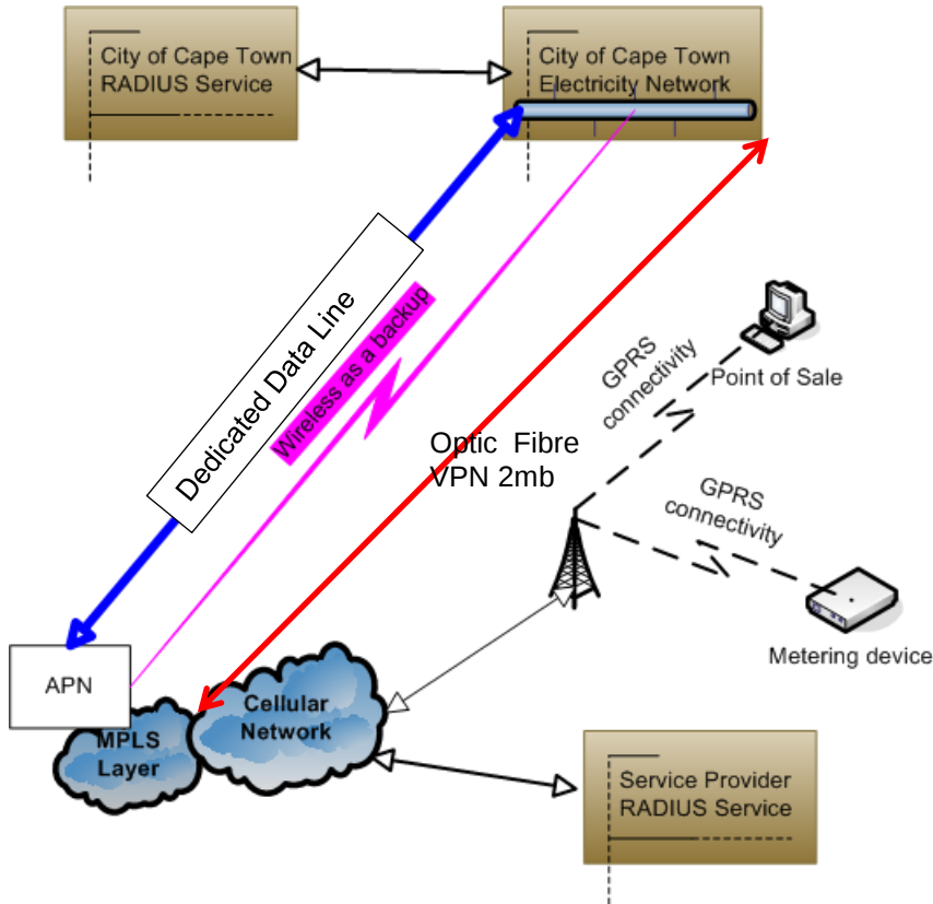
Figure 1. GPRS/EDGE/3G/HSDPA Data Interconnection Diagram, with RADIUS authentication
