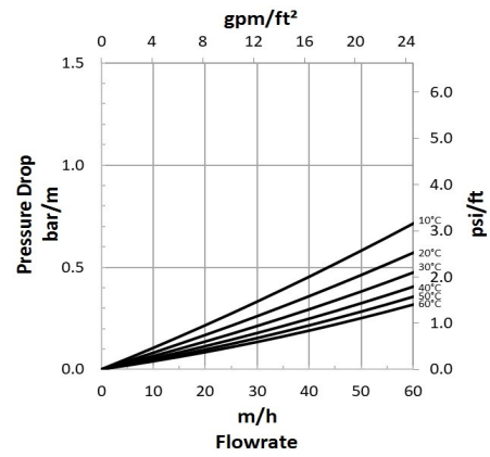
Figure 1: Pressure Drop
