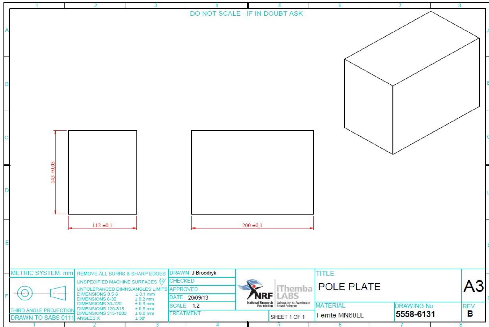
Figure 6: Drawing of the pole plate.
