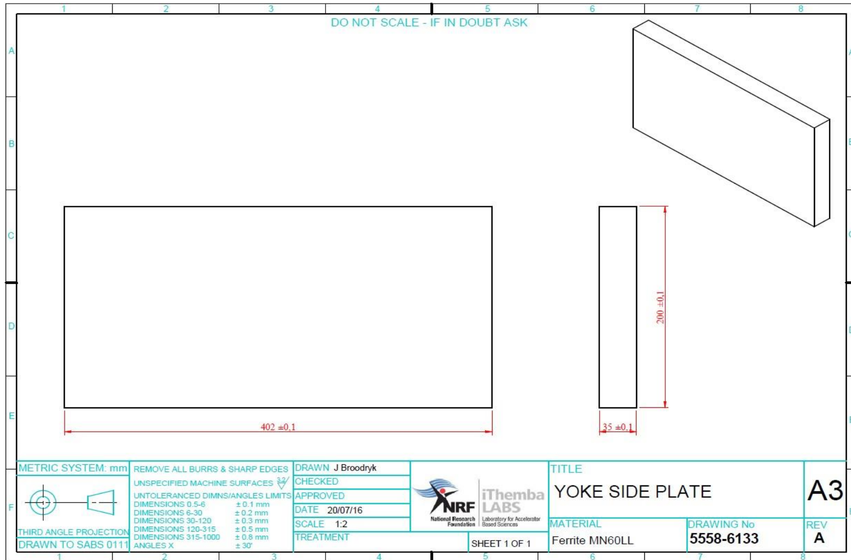
Figure 5: Drawing of a side yoke plate.
