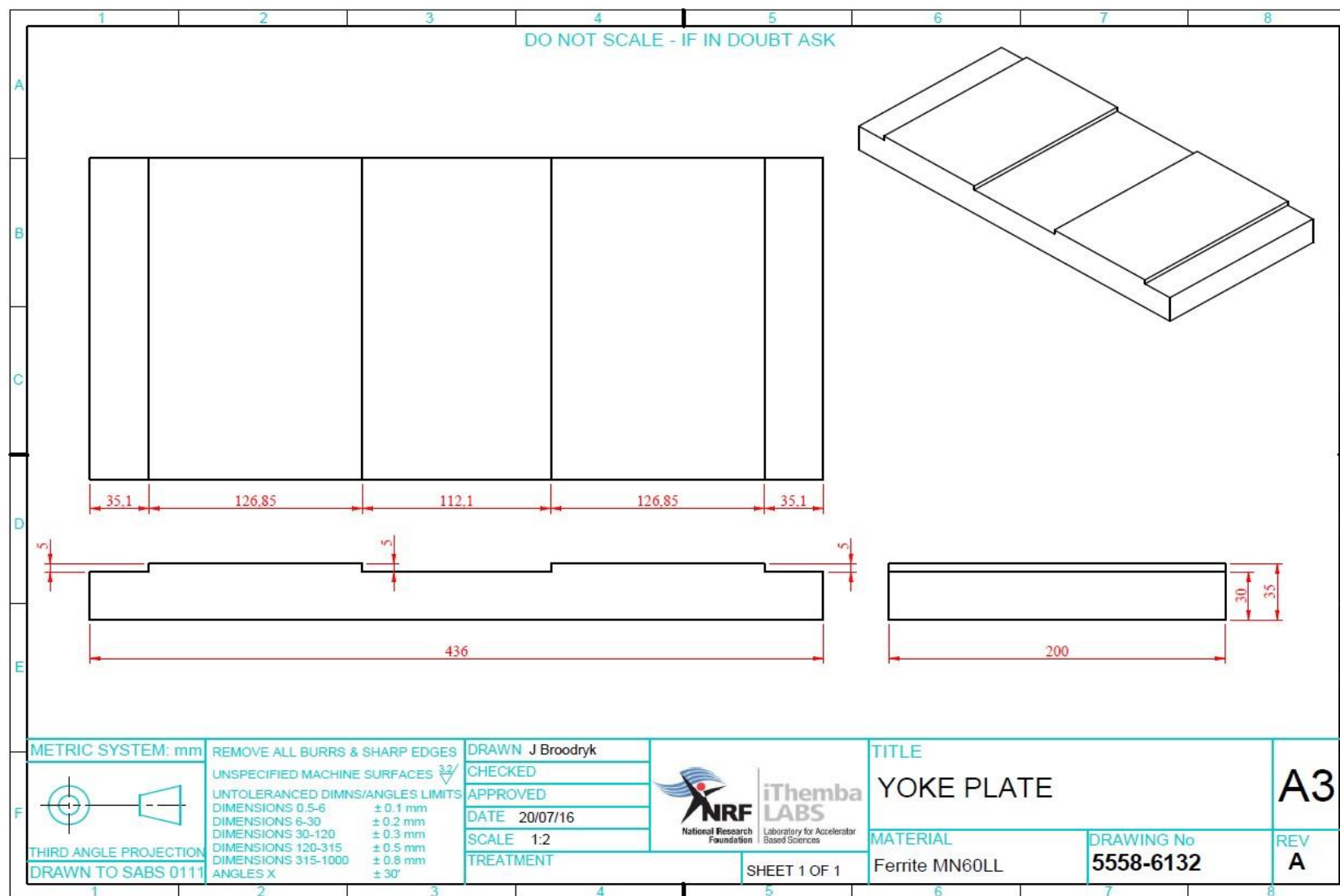
Figure 4: Drawing of a top and bottom yoke plate with the groove to insert the pole plate.
