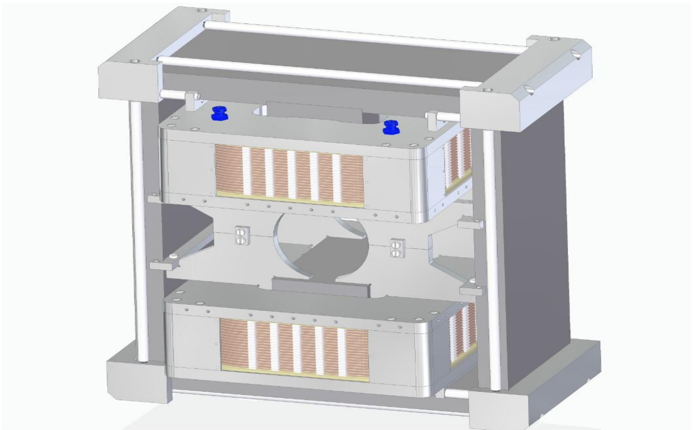
Figure 2: A 3-dimensional drawing of a sweeper magnet with coils.
