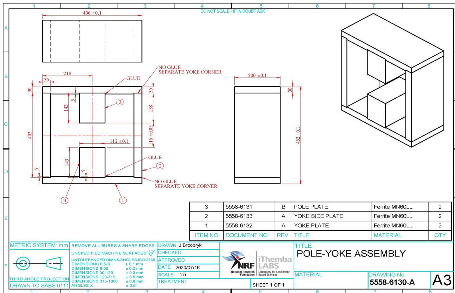
Figure 3: Drawing of a complete magnet assembly.
