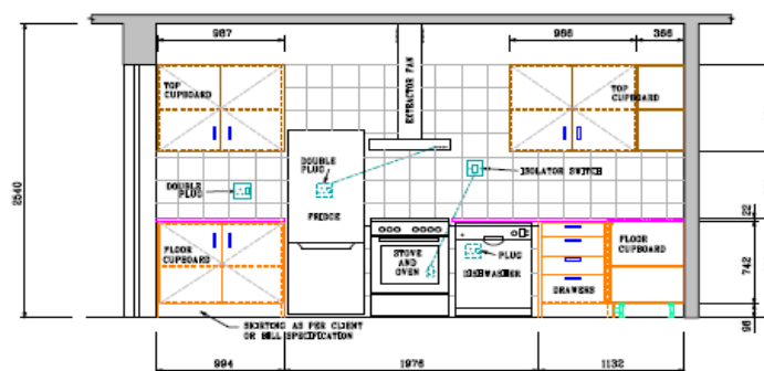
SECTION - 1
