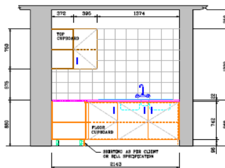
SECTION - 2
