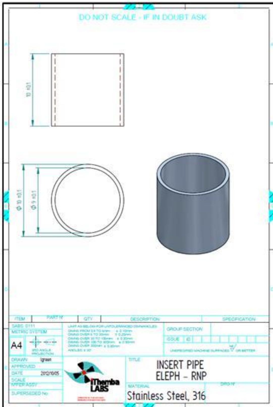
Drawing 1: Insert Pipe Eleph - RNP
