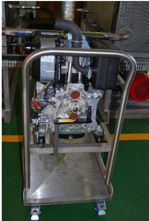
Pongolapoort dam: radial gate diesel driven standby hydraulic power pack
