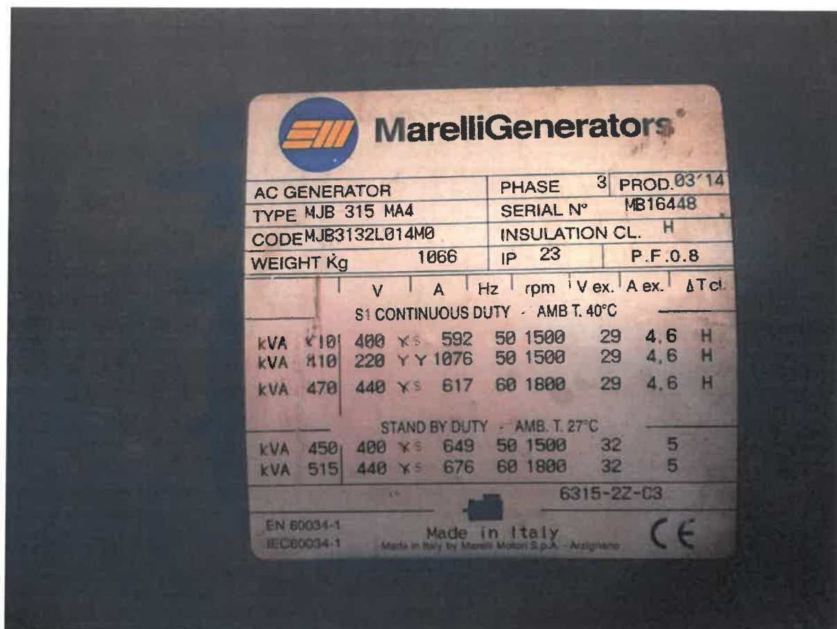
Image 5: Alternator nameplate
