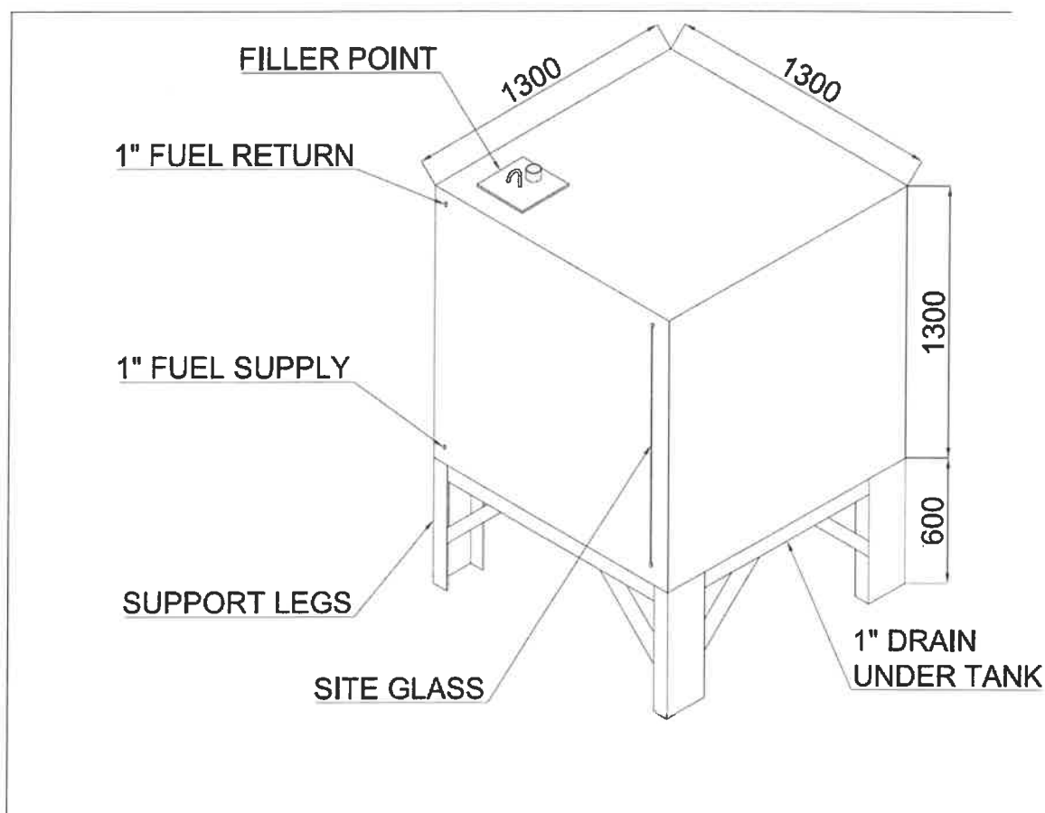
Image 6: Example of a typical freestanding fuel tank. Dimensions for the purposes of this project will differ.
