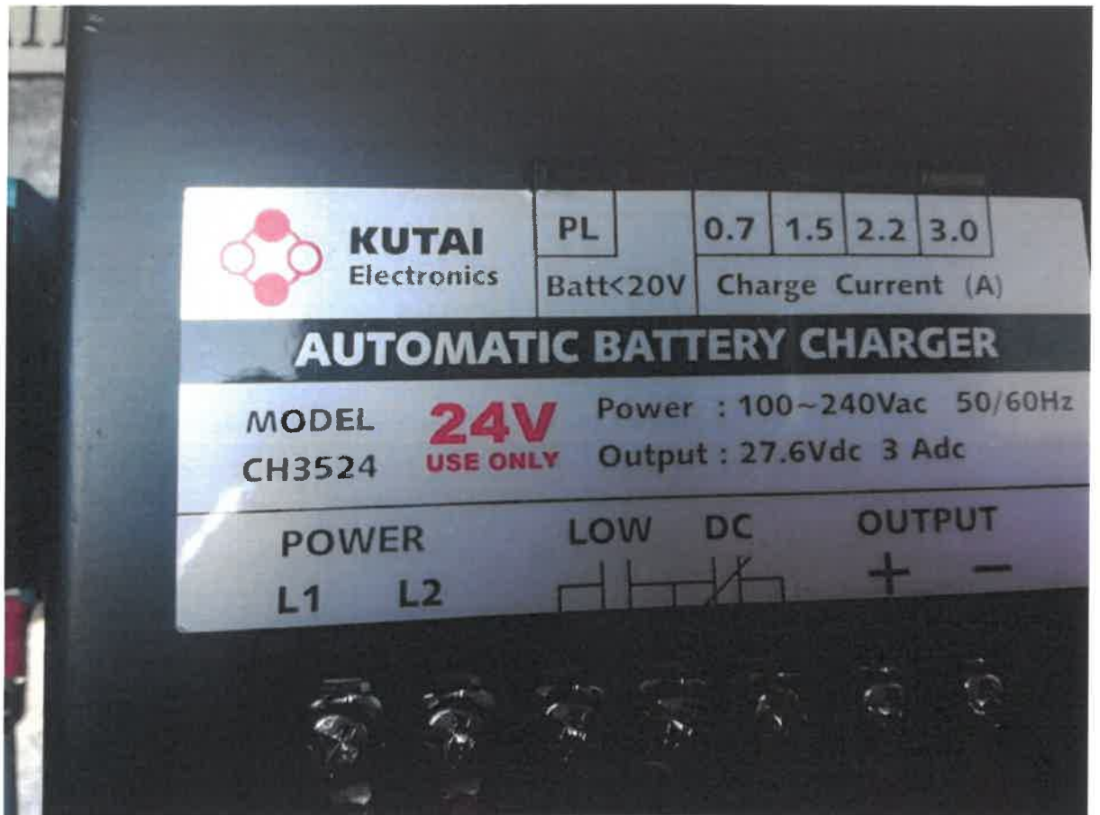
Image 4: Battery charger
