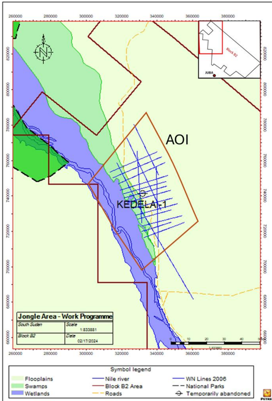
Figure 3 Physiographic map showing the location of Kedelai-1 well and legacy seismic lines in Block B2, South Sudan, highlighting the area of interest.
