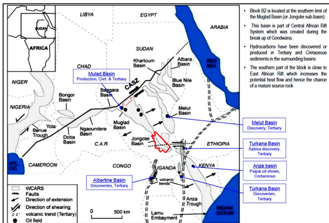
Figure 1: Map showing the location of the Muglad Basin and Sub-basins of Sudan as a part of the Central African Rift System. The red polygon represents the boundary of Block B2 in the Jonglei Sub-Basin. (Modified after Makeen Y.M 2021)
