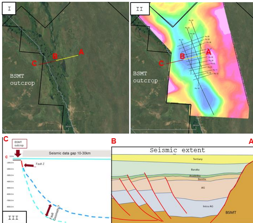
Figure 4 (I). Aerial Google Maps of the Study Area Showcasing the Outcropping Basement on the flanks of the Graben, (II). Basement depth map derived from gravity data. (III). cross section across the graben showing the extent of the seismic data.
