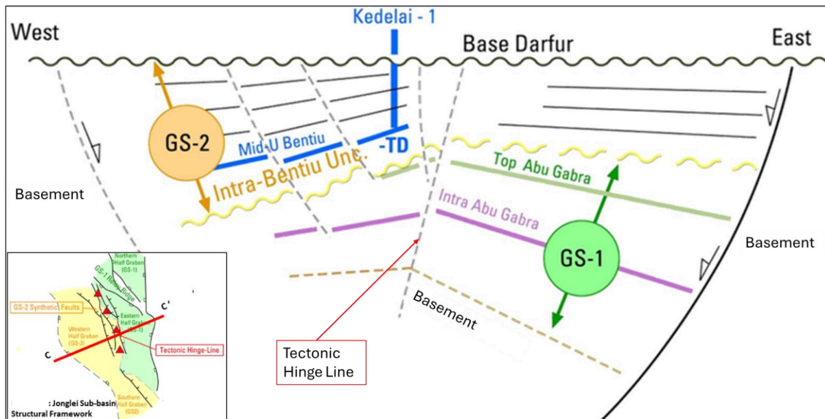
Figure 6: Schematic cross section of Jonglei sub basin representing the central part. (GS: Growth Sequence)
