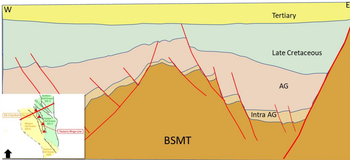
Figure 5 Schematic cross section of Jonglei Subbasin representing the Northern sector of the basin
