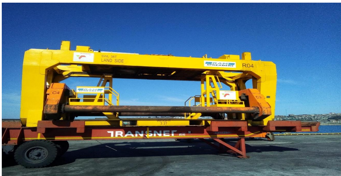
Figure 11: Revolver spreader
