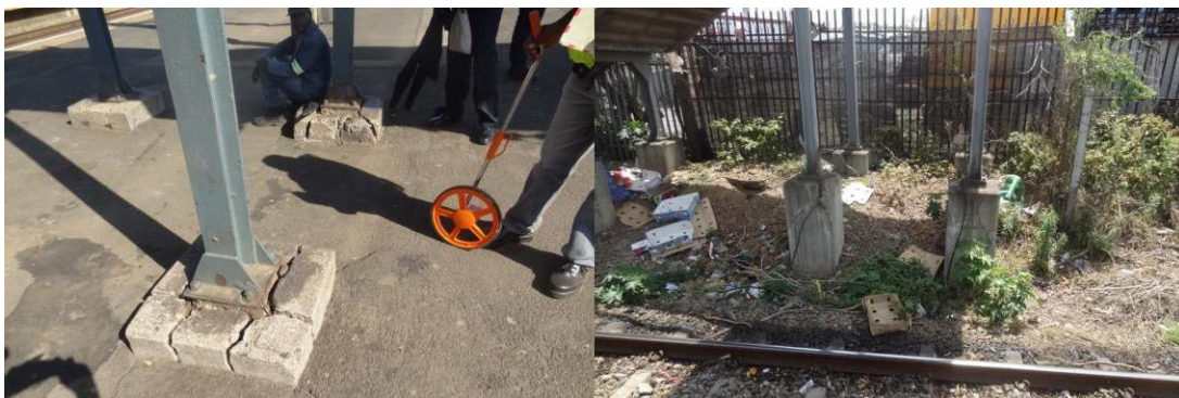
Figure 4 Foundation Defects
