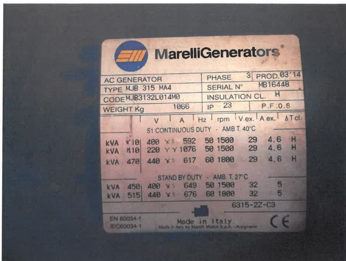
Image 5: Alternator nameplate
