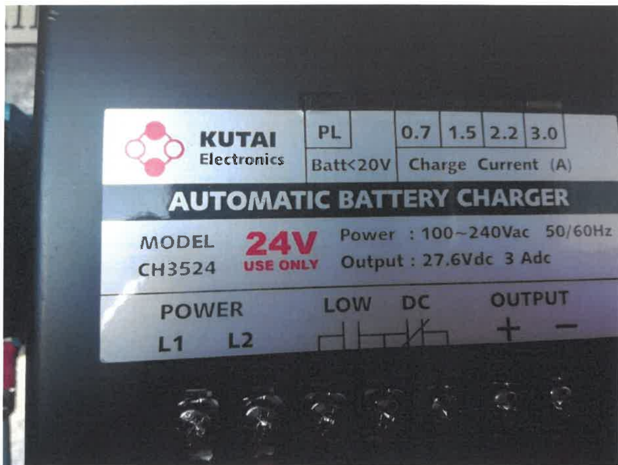
Image 4: Battery charger
