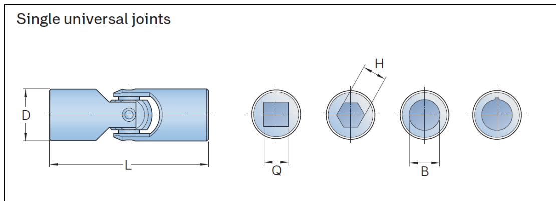
Figure 1: Typical Universal Joint Dimensions
