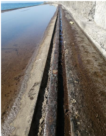
Figure 6: Corroded Rail
