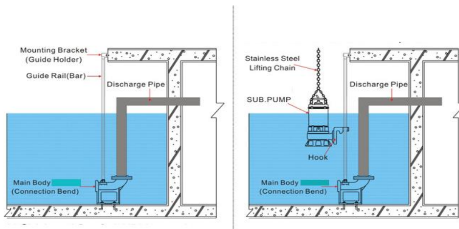
FIGURE 2: REFERENCE OF THE SUMPS AFTER COMPLETION OF WORKS
