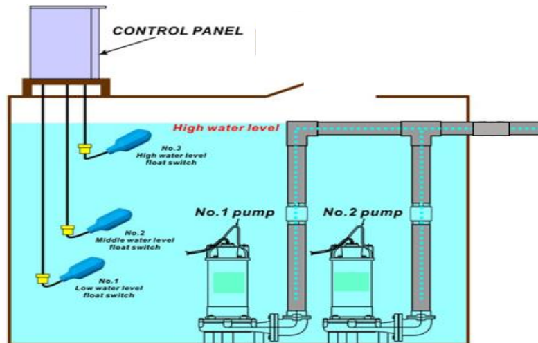
FIGURE 1: SUBMERSIBLE SEWAGE PUMPS ALTERNATIVE & PARALLEL OPERATION
